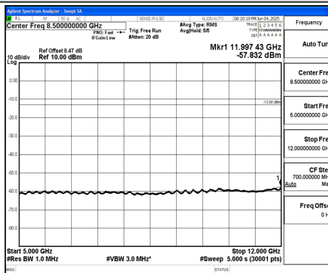
Band66-Stand-Alone-NaN-BPSK-132322-1@0-15kHz-5000-12000-5000~12000MHz@-57.83dBm--13-PASS
