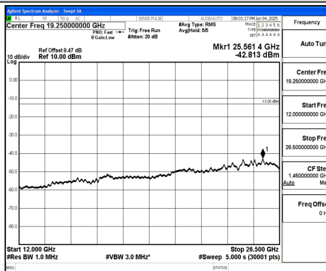
Band66-Stand-Alone-NaN-QPSK-132322-12@0-15kHz-12000-26500-12000~26500MHz@-42.81dBm--13-PASS
