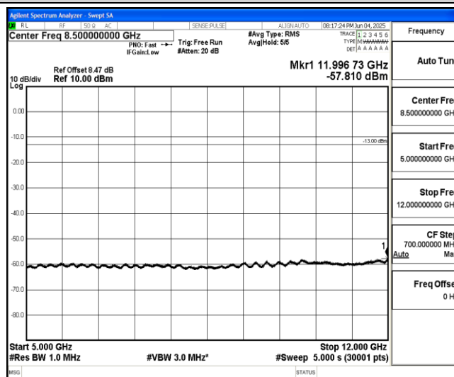
Band66-Stand-Alone-NaN-BPSK-132671-1@11-15kHz-5000-12000-5000~12000MHz@-57.81dBm--13-PASS
