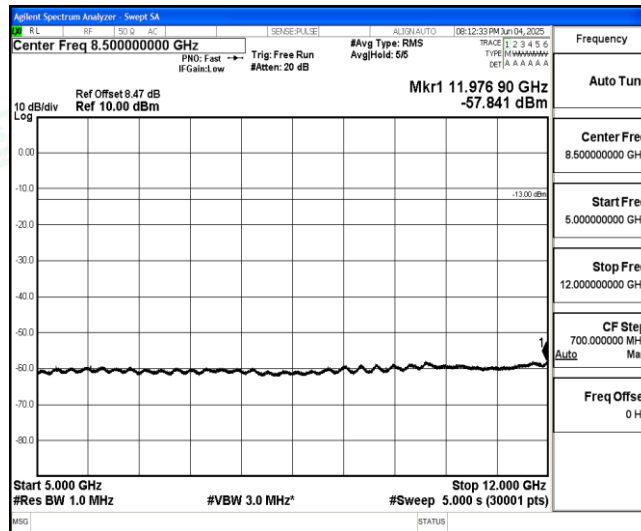
Band66-Stand-Alone-NaN-BPSK-132322-1@11-15kHz-5000-12000-5000~12000MHz@-57.84dBm--13-PASS
