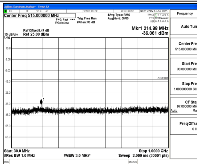
Band66-Stand-Alone-NaN-BPSK-131973-1@11-15kHz-30-1000-30~1000MHz@-36.06dBm--13-PASS
