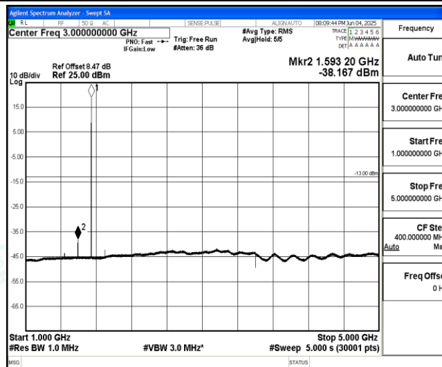
Band66-Stand-Alone-NaN-BPSK-132322-1@0-15kHz-1000-5000-1000~5000MHz@-38.17dBm--13-PASS
