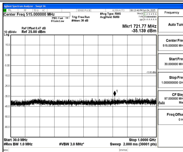
Band66-Stand-Alone-NaN-BPSK-132671-1@0-15kHz-30-1000-30~1000MHz@-35.14dBm--13-PASS
