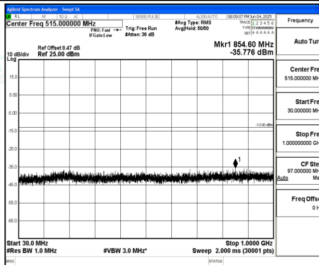
Band66-Stand-Alone-NaN-BPSK-132322-1@0-15kHz-30-1000-30~1000MHz@-35.78dBm--13-PASS
