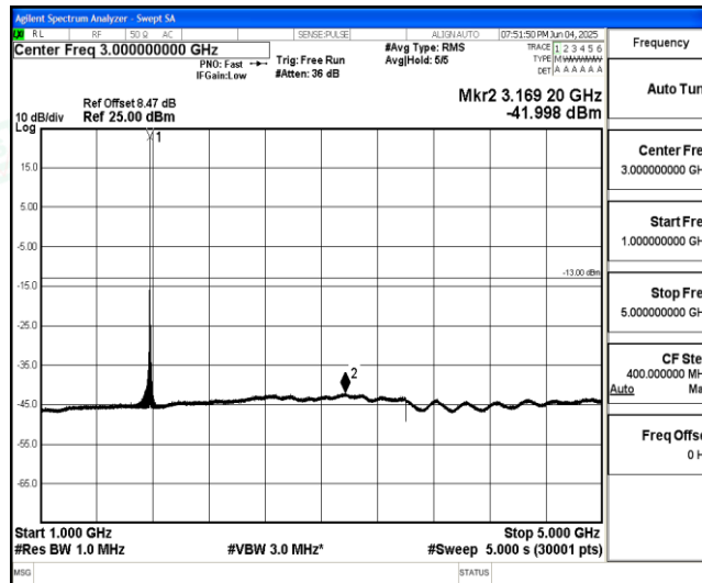
Band66-Stand-Alone-NaN-QPSK-132671-1@0-3.75kHz-1000-5000-1000~5000MHz@-42dBm--13-PASS
