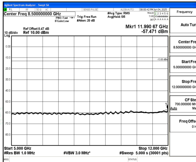
Band66-Stand-Alone-NaN-QPSK-132322-12@0-15kHz-5000-12000-5000~12000MHz@-57.47dBm--13-PASS
