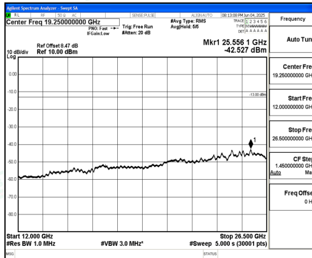
Band66-Stand-Alone-NaN-BPSK-132322-1@11-15kHz-12000-26500-12000~26500MHz@-42.53dBm--13-PASS
