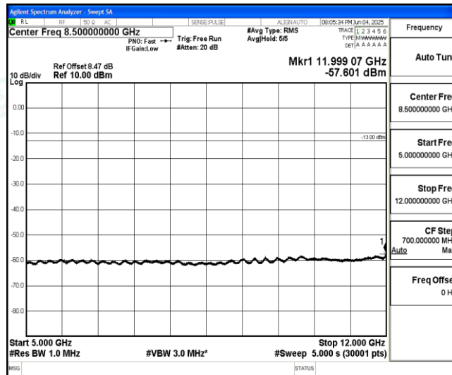
Band66-Stand-Alone-NaN-BPSK-131973-1@0-15kHz-5000-12000-5000~12000MHz@-57.6dBm--13-PASS
