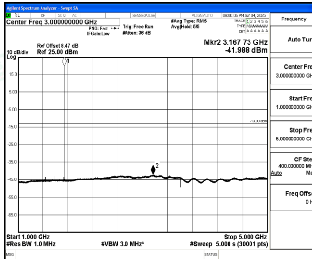
Band66-Stand-Alone-NaN-QPSK-132322-12@0-15kHz-1000-5000-1000~5000MHz@-41.99dBm--13-PASS
