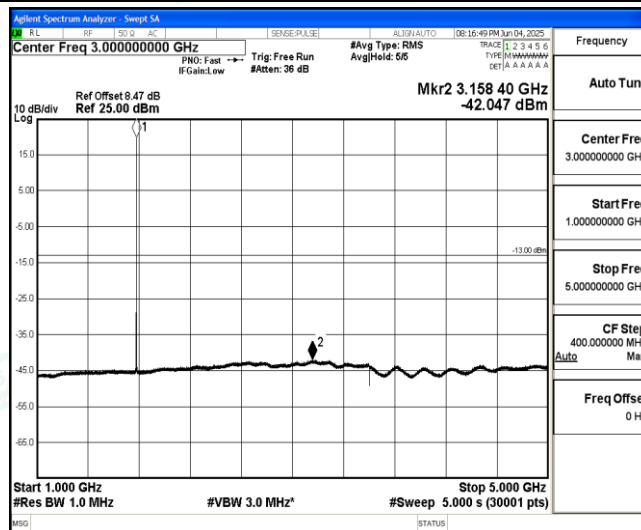
Band66-Stand-Alone-NaN-BPSK-132671-1@11-15kHz-1000-5000-1000~5000MHz@-42.05dBm--13-PASS
