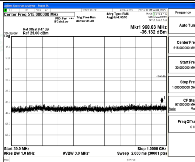
Band66-Stand-Alone-NaN-BPSK-132671-1@11-15kHz-30-1000-30~1000MHz@-36.13dBm--13-PASS
