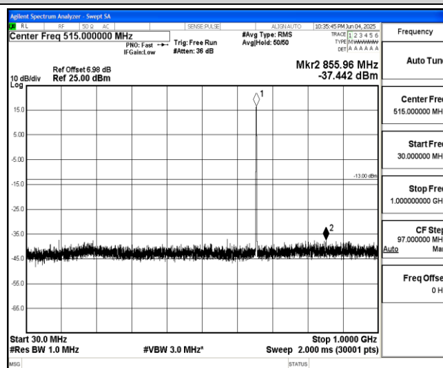
Band71-Stand-Alone-NaN-BPSK-133123-1@11-15kHz-30-1000-30~1000MHz@-37.44dBm--13-PASS
