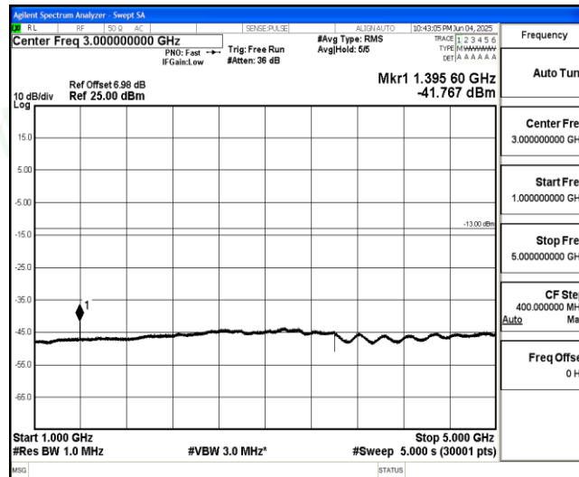
Band71-Stand-Alone-NaN-BPSK-133471-1@0-15kHz-1000-5000-1000~5000MHz@-41.77dBm--13-PASS
