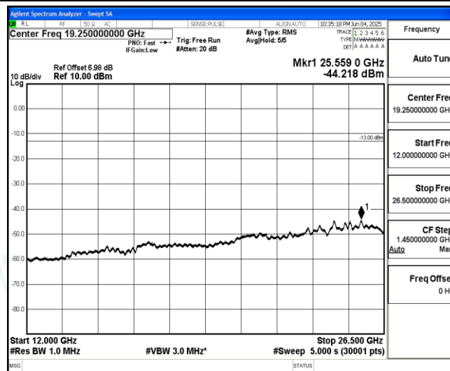
Band71-Stand-Alone-NaN-BPSK-133123-1@0-15kHz-12000-26500-12000~26500MHz@-44.22dBm--13-PASS
