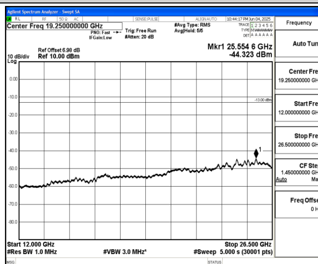
Band71-Stand-Alone-NaN-BPSK-133471-1@0-15kHz-12000-26500-12000~26500MHz@-44.32dBm--13-PASS
