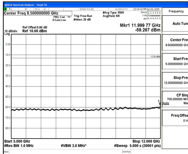
Band71-Stand-Alone-NaN-BPSK-133123-1@0-15kHz-5000-12000-5000~12000MHz@-59.27dBm--13-PASS
