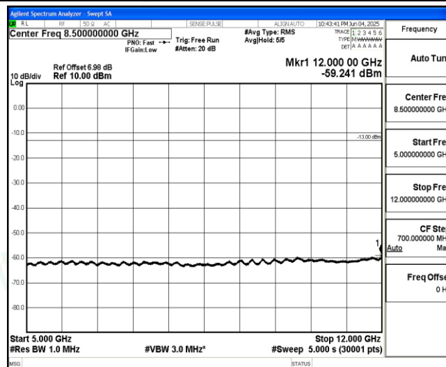
Band71-Stand-Alone-NaN-BPSK-133471-1@0-15kHz-5000-12000-5000~12000MHz@-59.24dBm--13-PASS
