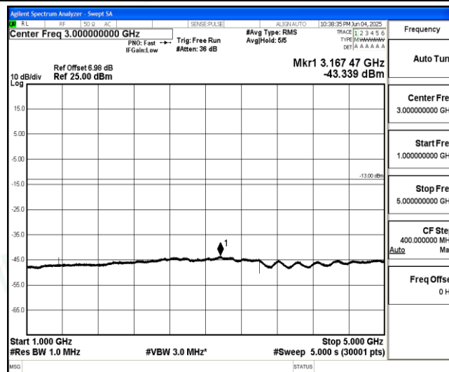
Band71-Stand-Alone-NaN-BPSK-133297-1@0-15kHz-1000-5000-1000~5000MHz@-43.34dBm--13-PASS
