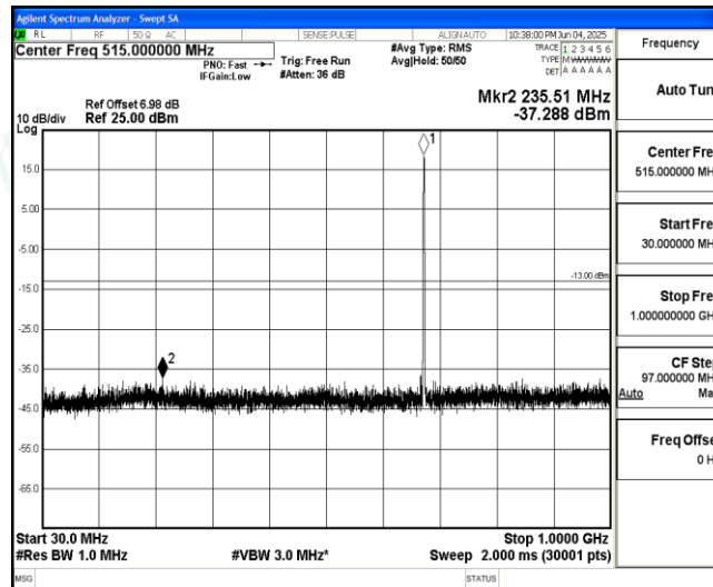
Band71-Stand-Alone-NaN-BPSK-133297-1@0-15kHz-30-1000-30~1000MHz@-37.29dBm--13-PASS
