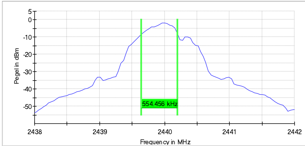
6 dB Bandwidth, Ch 17
