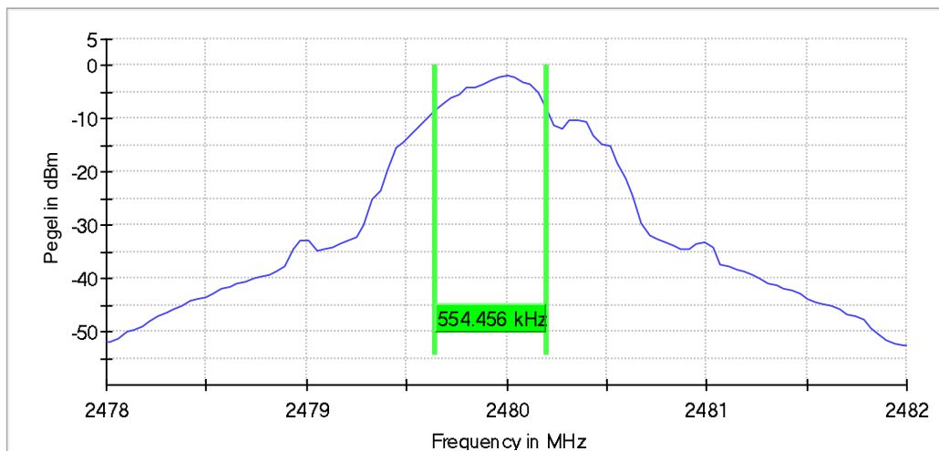
6 dB Bandwidth, Ch 39
