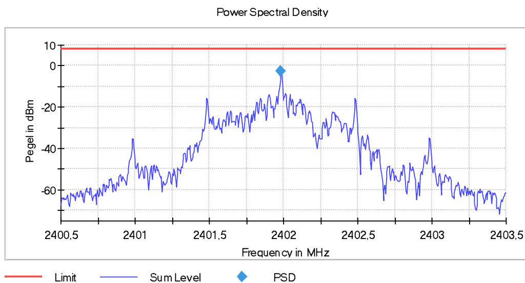
Power Spectral Density, Ch 37
