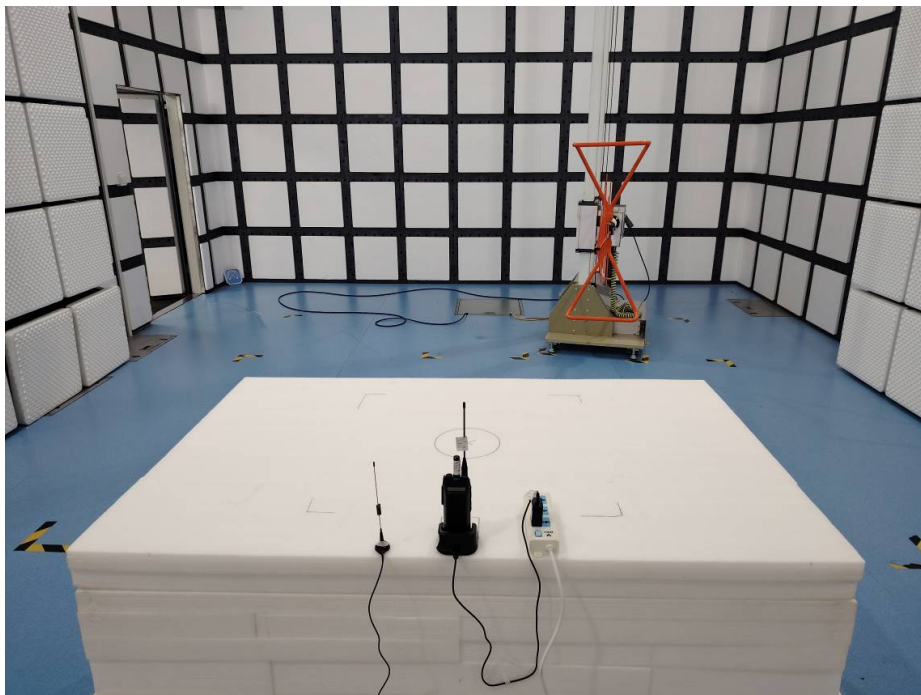
Radiation Emission - Back View (Below 1GHz)
