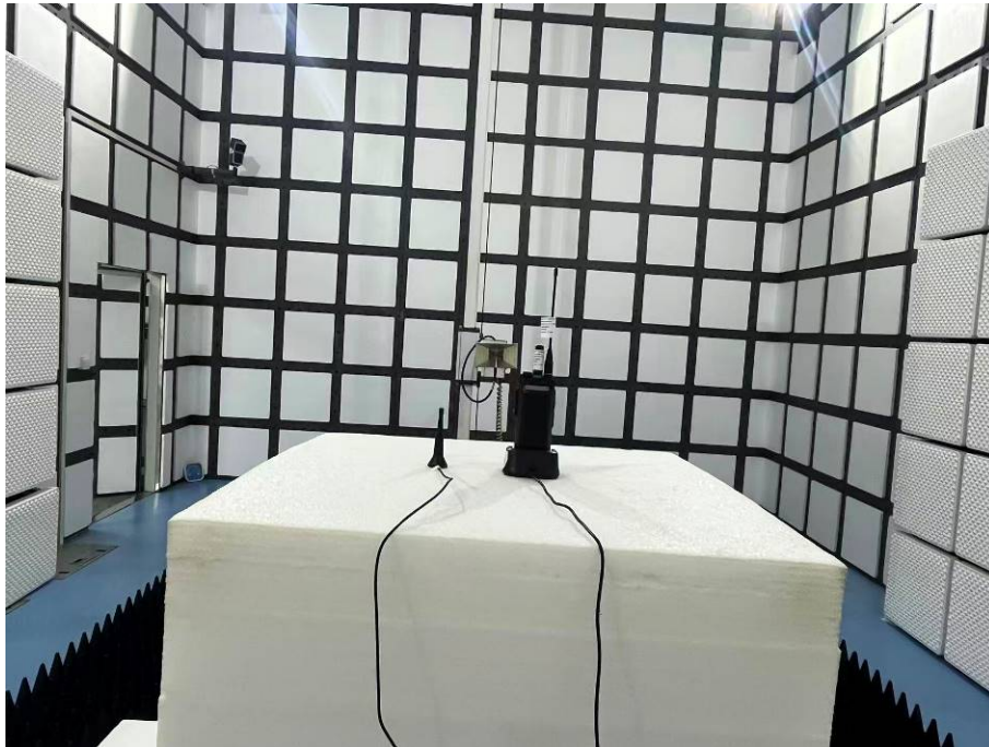
Radiation Emission - Back View (Above 1GHz)
