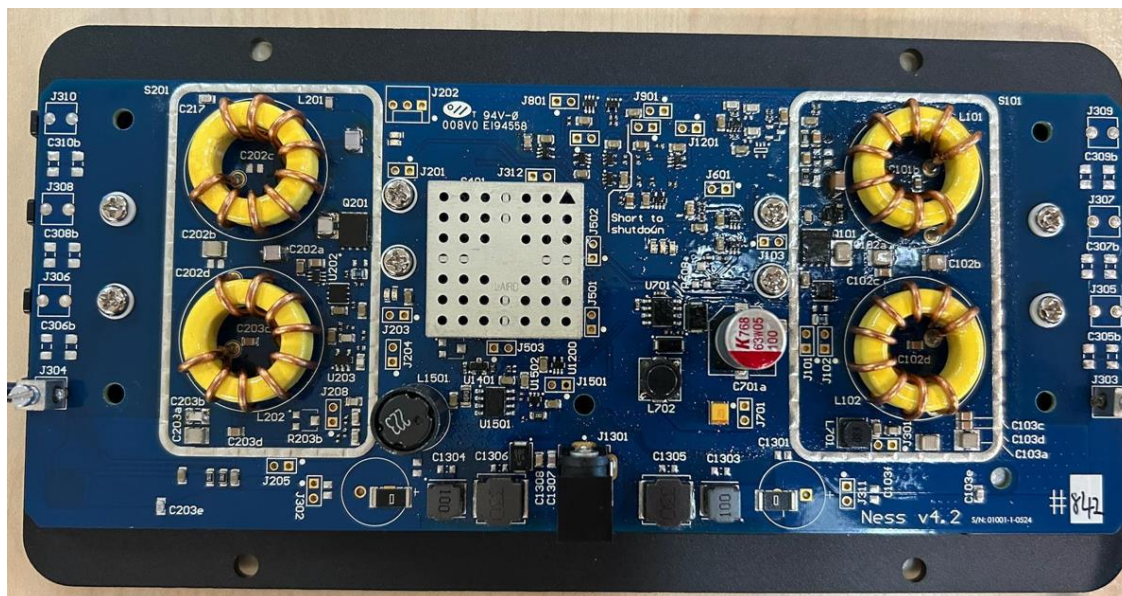
EUT – Rear side (with metal plate)
