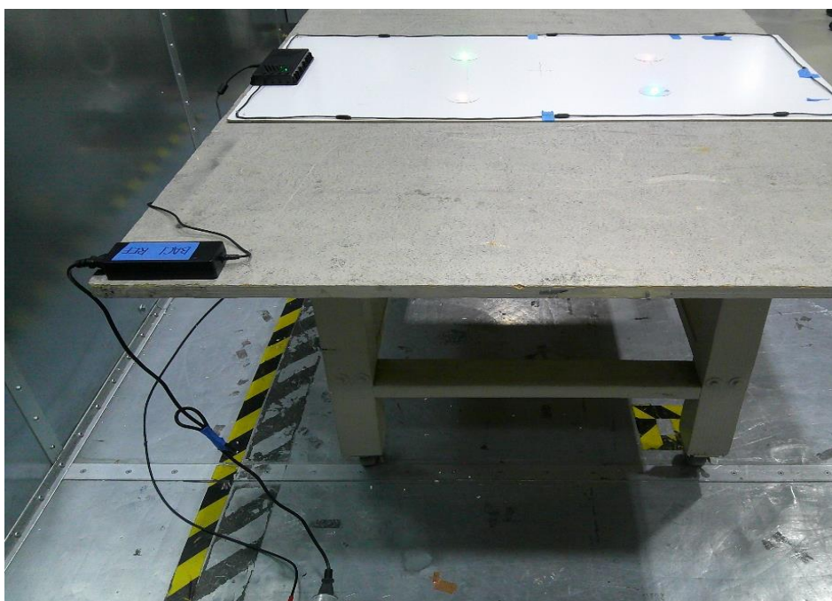
AC Line, Side View
