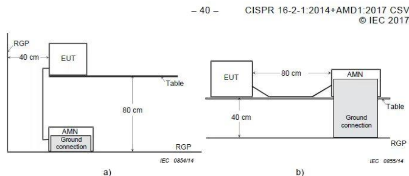
Figure 10 – Arrangement of EUT and AMN at 40 cm distance, with a) vertical RGP and b) horizontal RGP
