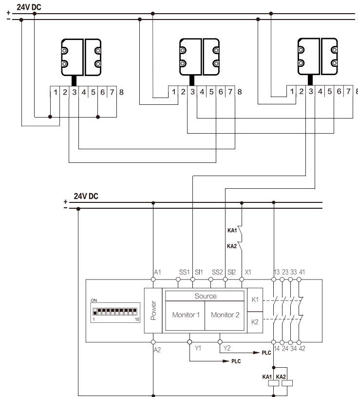
Example Diagram 3: Using multiple ENQMT20/ENQFT20 non-contact safety switches in cascade connect, with DNSC31S safety relay, dual channel detection, automatic reset
