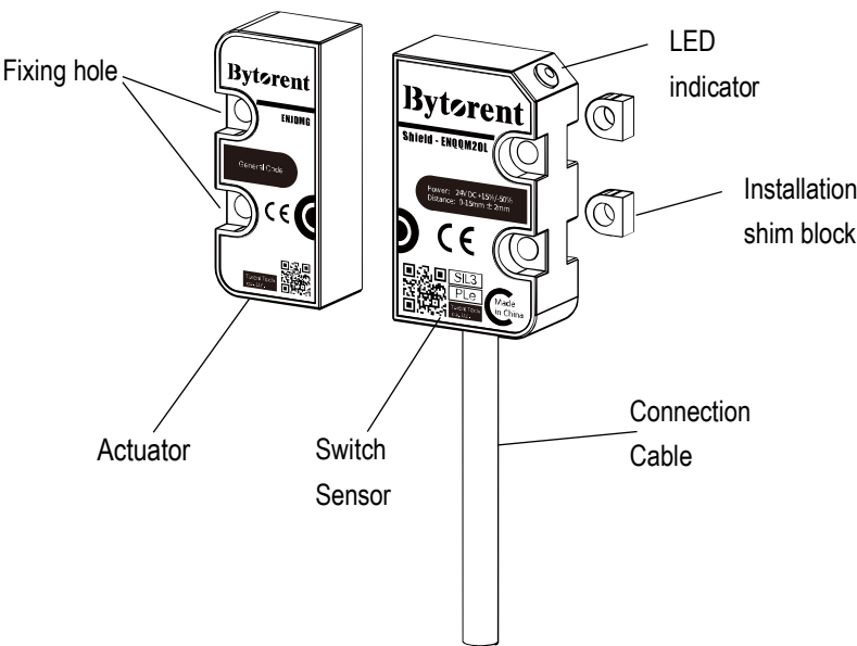
Switch sensor with Actuator (Front side)
