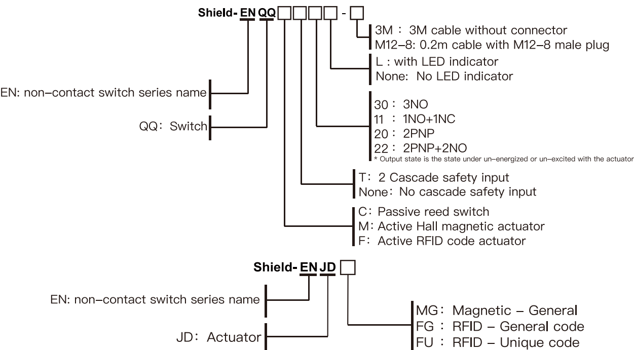
Sensor model and detailed description (the following output states are all states without power or induction excitation)
