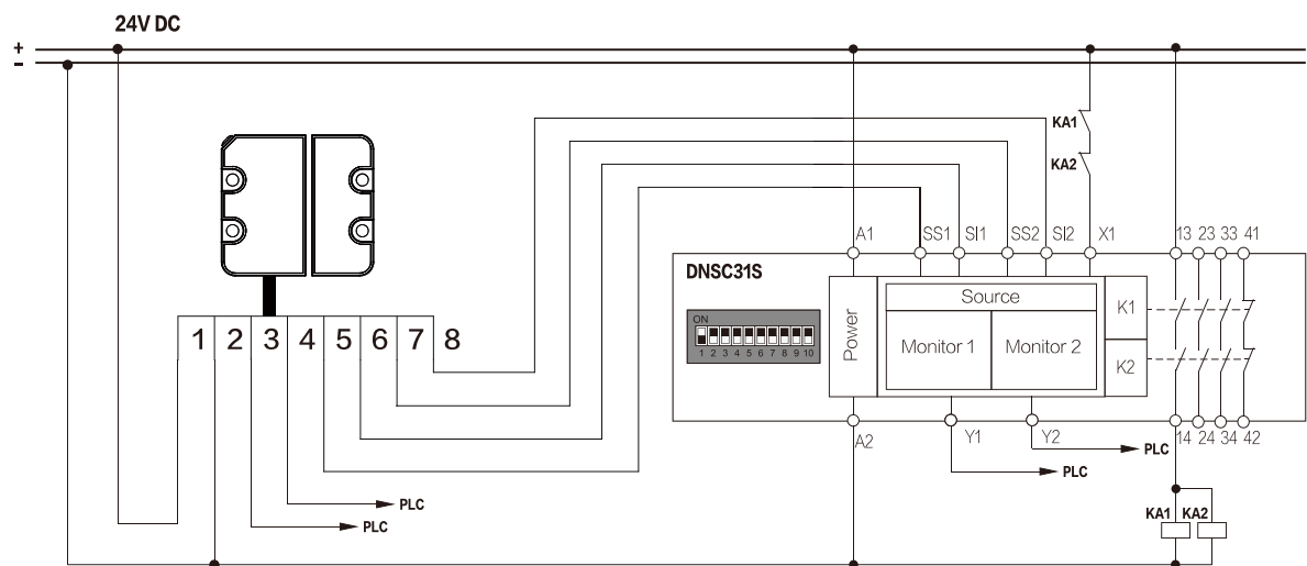
Example Diagram 1: Using ENQQF22L-3m RFID non-contact safety switch with DNSC31S safety relay, dual channels, automatically reset
