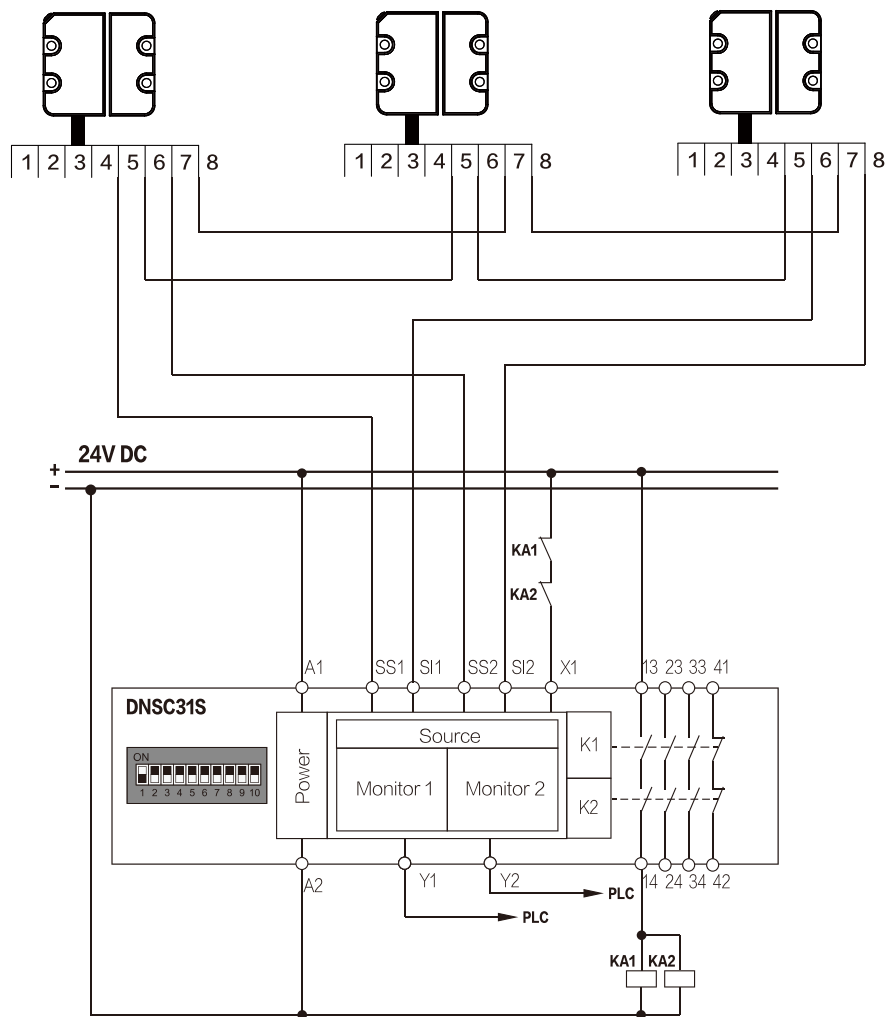
Example Diagram 2: Using multiple ENQQC30-3m non-contact safety switches in series cascade, with DNSC31S safety relay, dual channel detection, automatic reset
