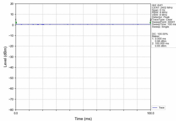
2M_LCH_2402MHz_Ant1_NTNV
