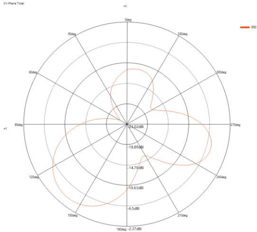
XY-Plane Total
