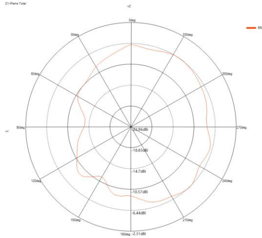
ZY-Plane Total
