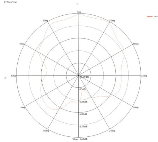
ZY-Plane Total
