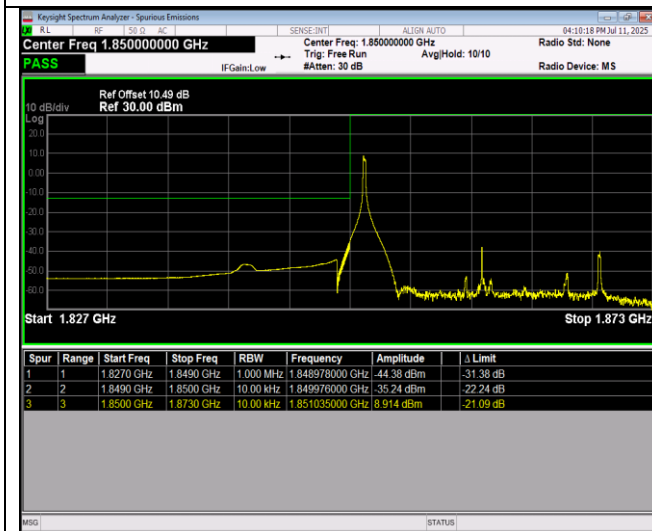
Band25-20MHz-64QAM-26140-100RB#0
