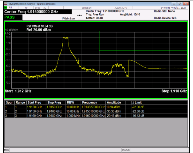
Band25-1.4MHz-16QAM-26683-6RB#0
