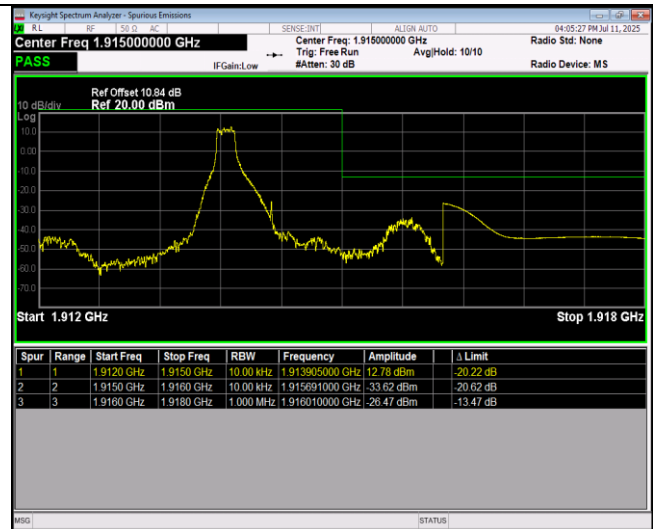
Band25-1.4MHz-QPSK-26683-6RB#0
