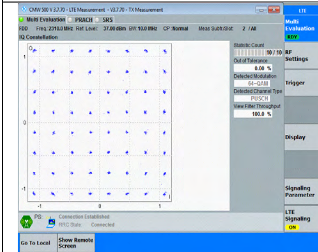
Band30-10MHz-64QAM-27710-50RB#0-PASS
