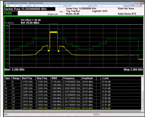
Band30-5MHz-64QAM-27735-1RB#24-PASS
