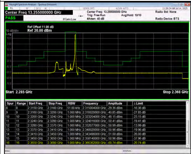
Band30-5MHz-16QAM-27735-1RB#0-PASS
