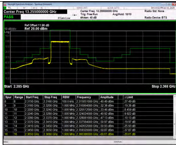
Band30-10MHz-64QAM-27710-1RB#49-PASS
