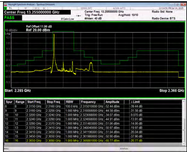
Band30-10MHz-64QAM-27710-50RB#0-PASS
