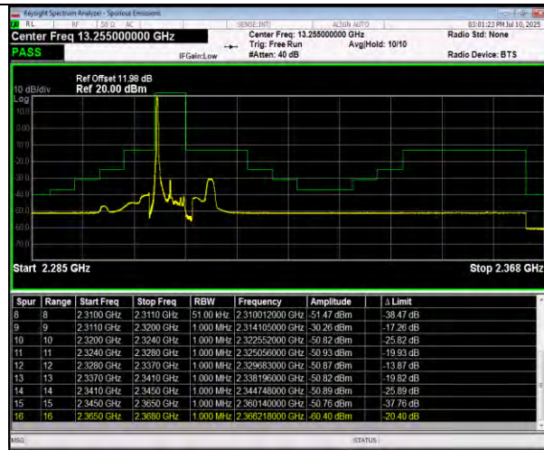
Band30-5MHz-QPSK-27685-25RB#0-PASS
