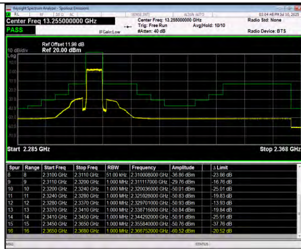
Band30-5MHz-64QAM-27685-1RB#24-PASS
