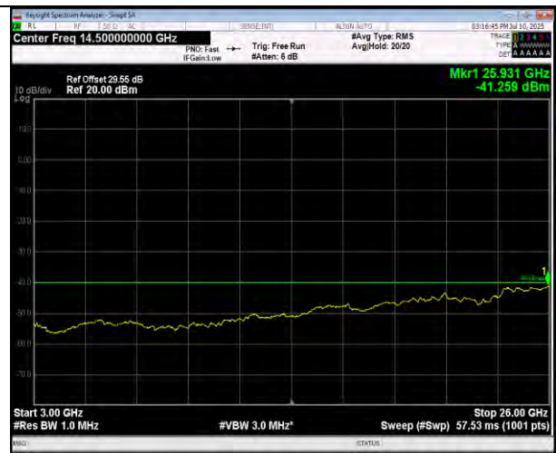
Band30-5MHz-QPSK-27735-1RB#24-3000~26000-PASS
