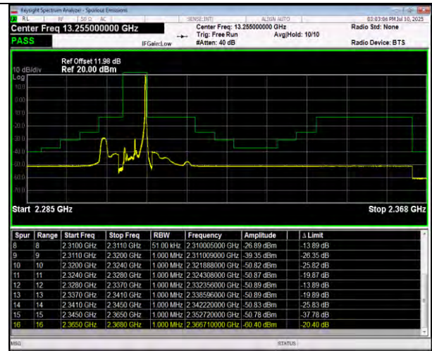
Band30-5MHz-64QAM-27685-1RB#0-PASS
