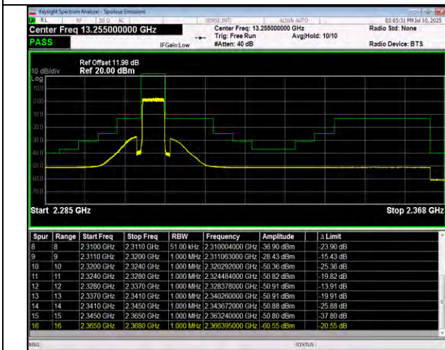
Band30-5MHz-16QAM-27685-25RB#0-PASS
