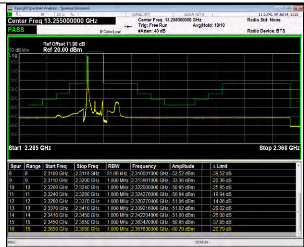
Band30-5MHz-64QAM-27685-25RB#0-PASS
