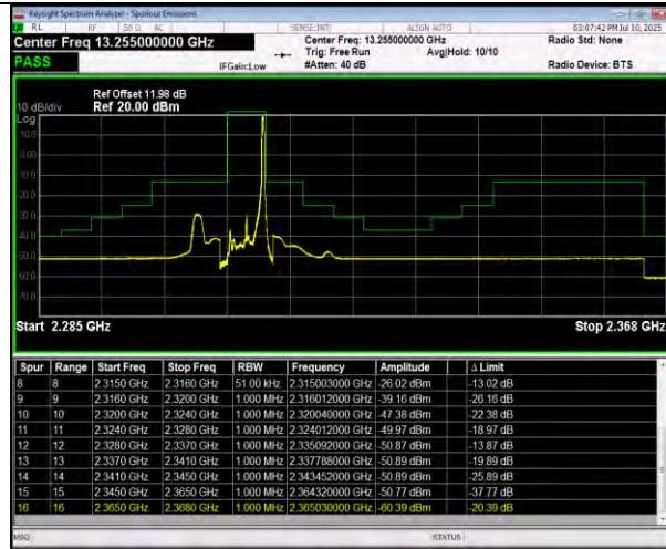
Band30-5MHz-64QAM-27735-1RB#0-PASS
