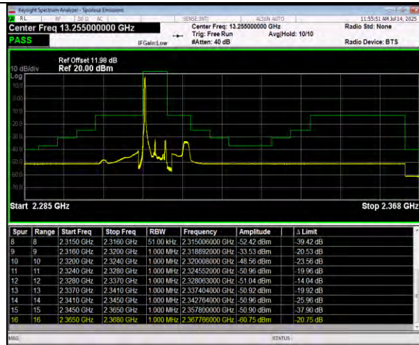
Band30-5MHz-64QAM-27735-25RB#0-PASS
