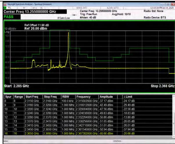
Band30-10MHz-16QAM-27710-1RB#0-PASS
