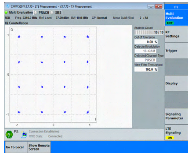
Band30-10MHz-16QAM-27710-50RB#0-PASS
