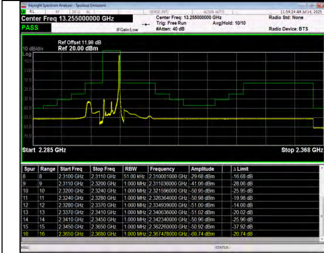
Band30-5MHz-16QAM-27685-1RB#0-PASS
