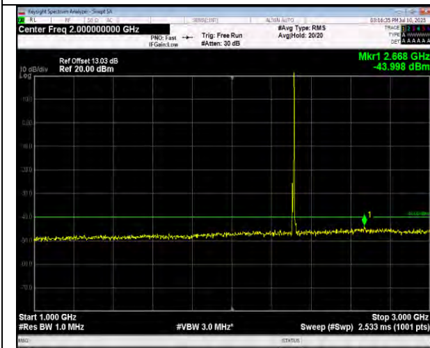
Band30-5MHz-QPSK-27735-1RB#24-1000~3000-PASS
