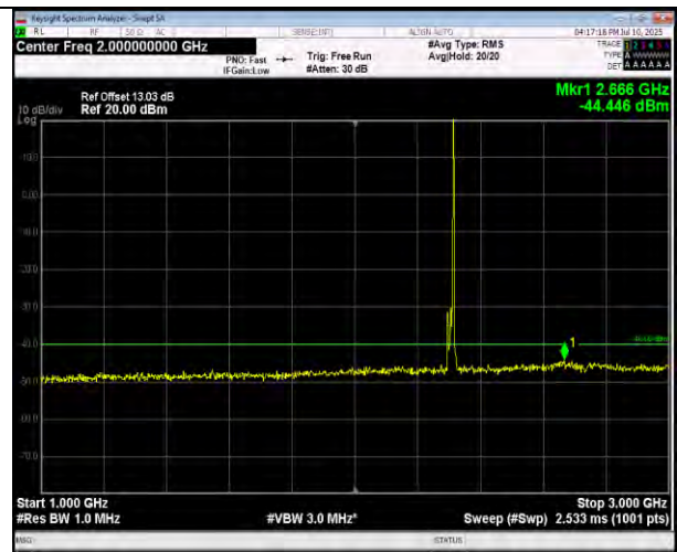
Band30-10MHz-16QAM-27710-1RB#49-1000~3000-PASS
