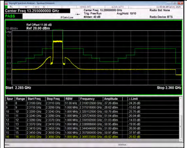
Band30-5MHz-16QAM-27685-1RB#24-PASS
