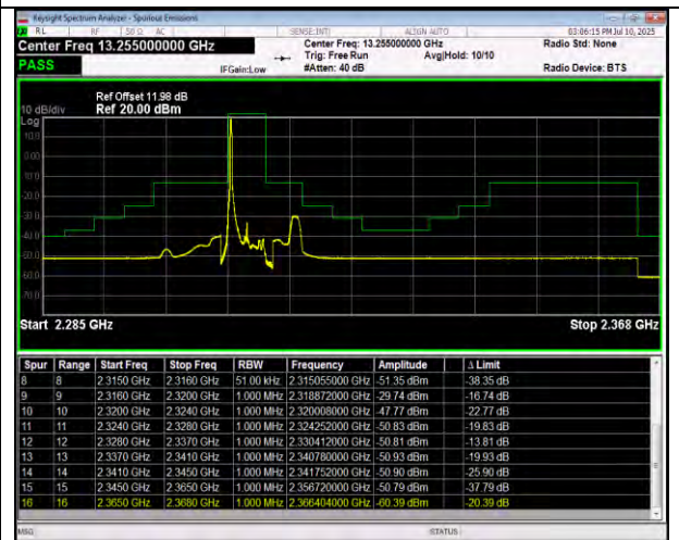
Band30-5MHz-QPSK-27735-1RB#0-PASS
