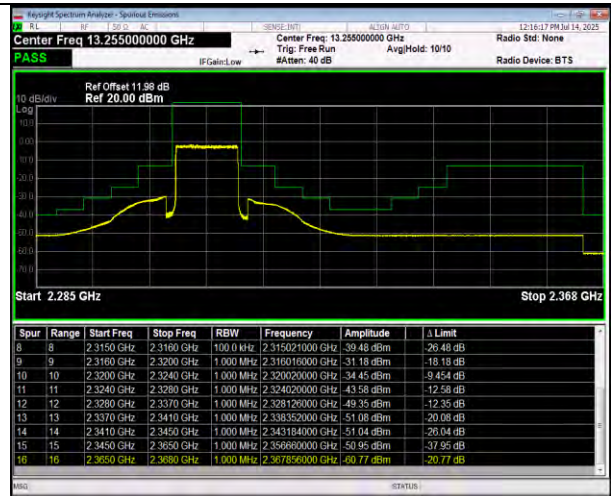
Band30-10MHz-16QAM-27710-1RB#49-PASS
