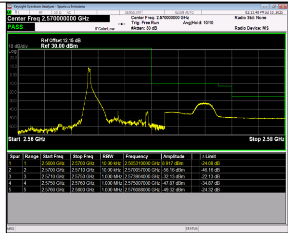
Band7-5MHz-64QAM-21425-25RB#0
