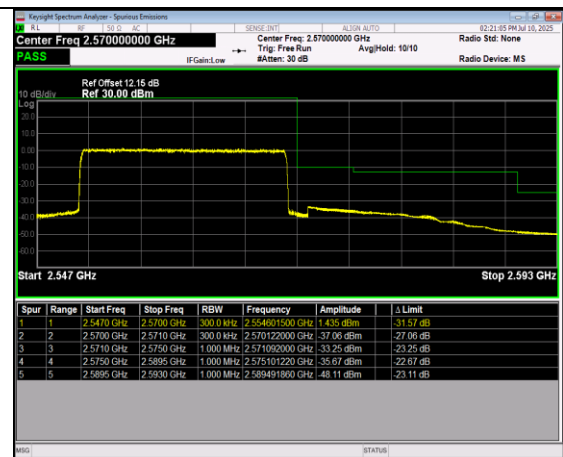
Band7-20MHz-64QAM-21350-100RB#0
