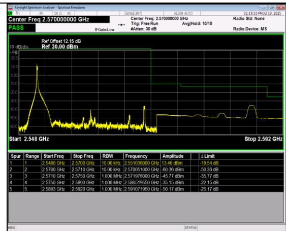
Band7-20MHz-QPSK-21350-100RB#0
