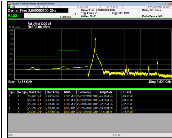
Band7-20MHz-QPSK-20850-100RB#0
