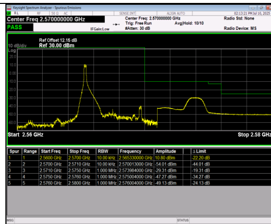
Band7-5MHz-QPSK-21425-25RB#0
