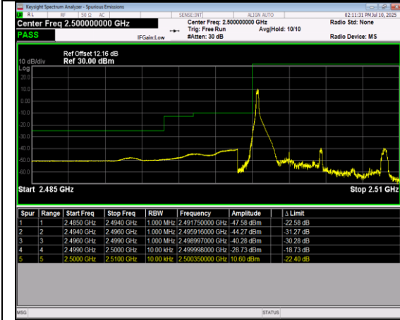
Band7-5MHz-64QAM-20775-25RB#0
