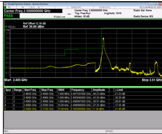
Band7-5MHz-QPSK-20775-25RB#0
