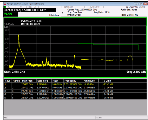
Band7-20MHz-16QAM-21350-100RB#0
