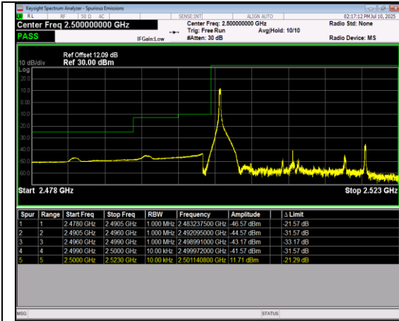
Band7-20MHz-16QAM-20850-100RB#0
