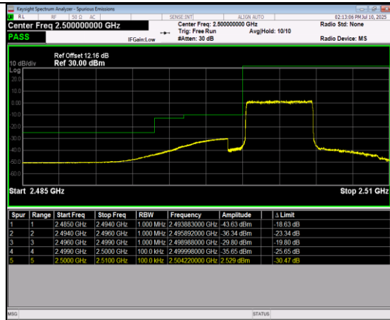
Band7-5MHz-64QAM-21425-1RB#24
