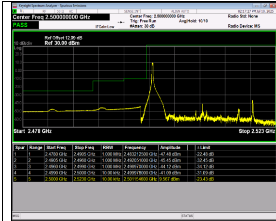
Band7-20MHz-64QAM-20850-100RB#0
