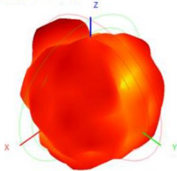
2450.0MHz H+V, Eff: 54.5%
