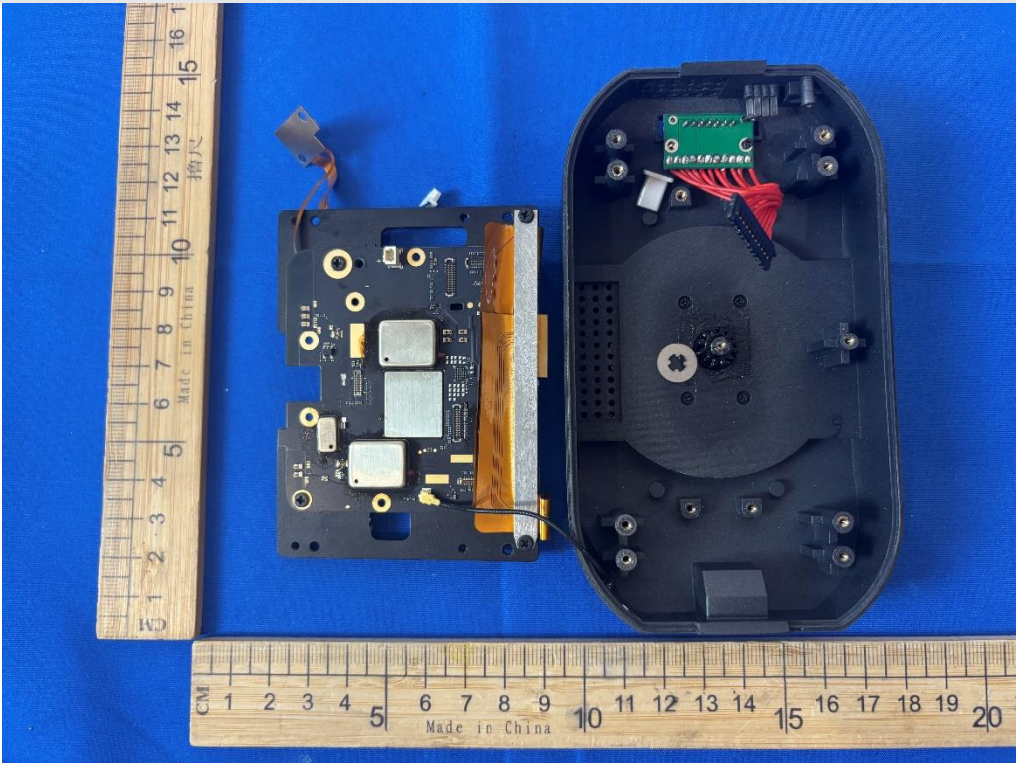
Internal View of EUT-31
