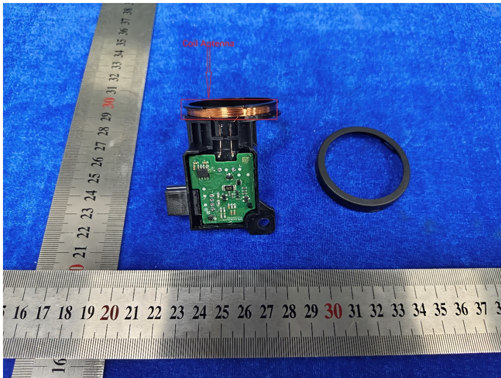
Photo 8: Internal View for 125kHz Antenna
