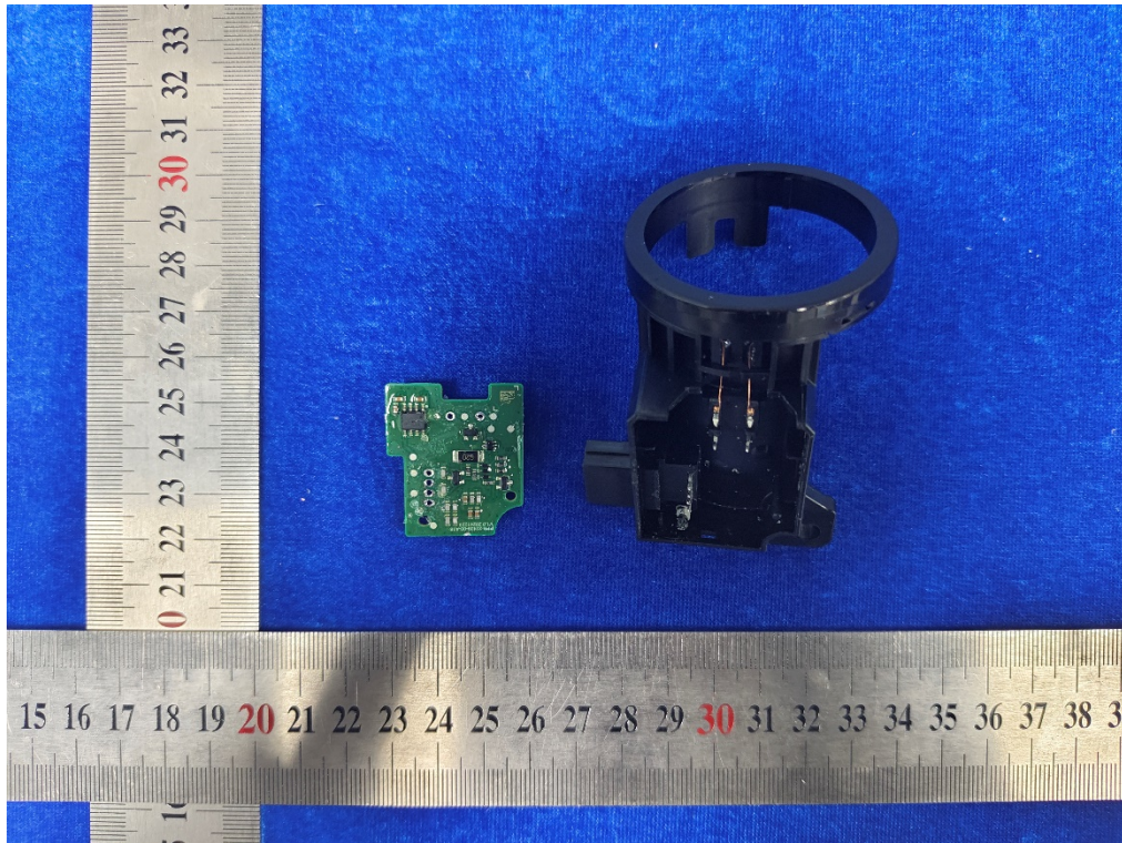
Photo 3: Internal View for 2.4G-WiFi/BLE Antenna
