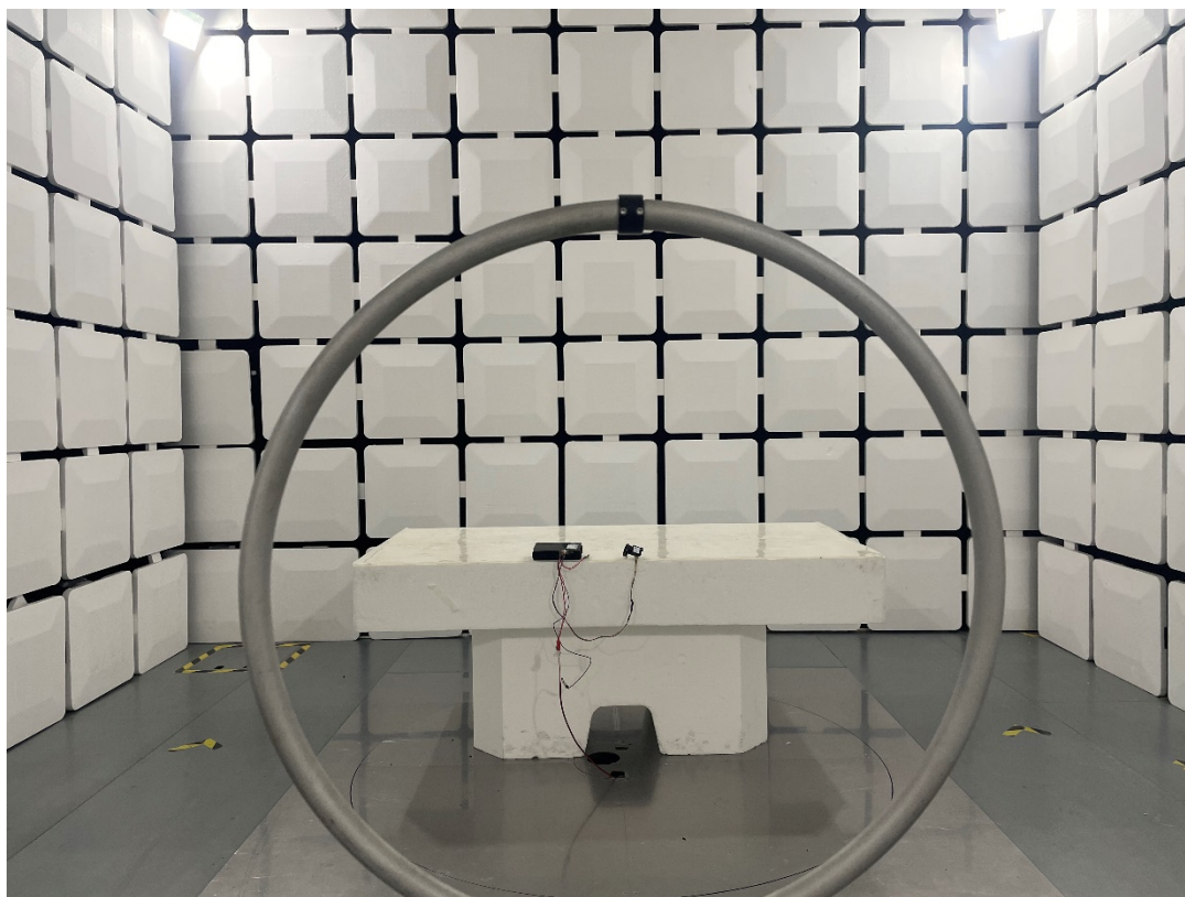
Description: Radiated Emission Test Setup for 9kHz-30MHz
