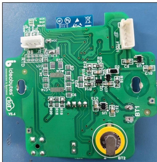
Main PCB Rear View
