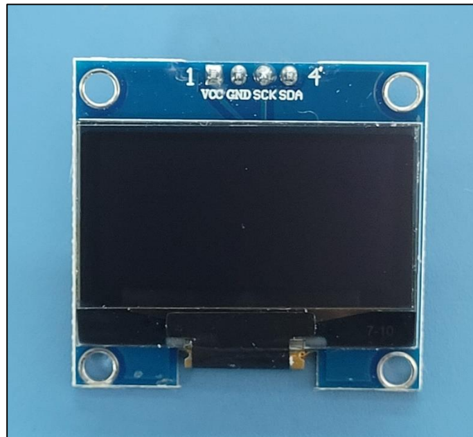
Display PCB Front View
