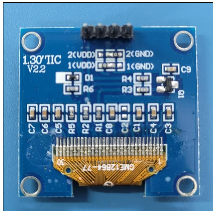
Display PCB Rear View
