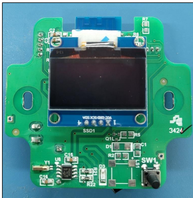
Main PCB Front View
