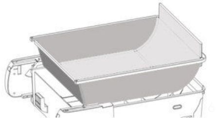
Remove the silicone pad upwards
