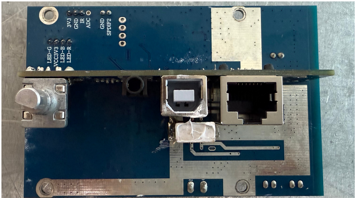
Main PCB Rear
