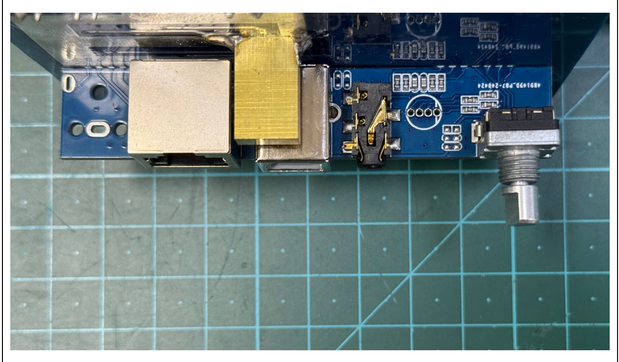
Sub PCB Front
