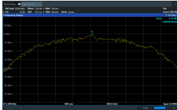
GFSK on Channel 01
