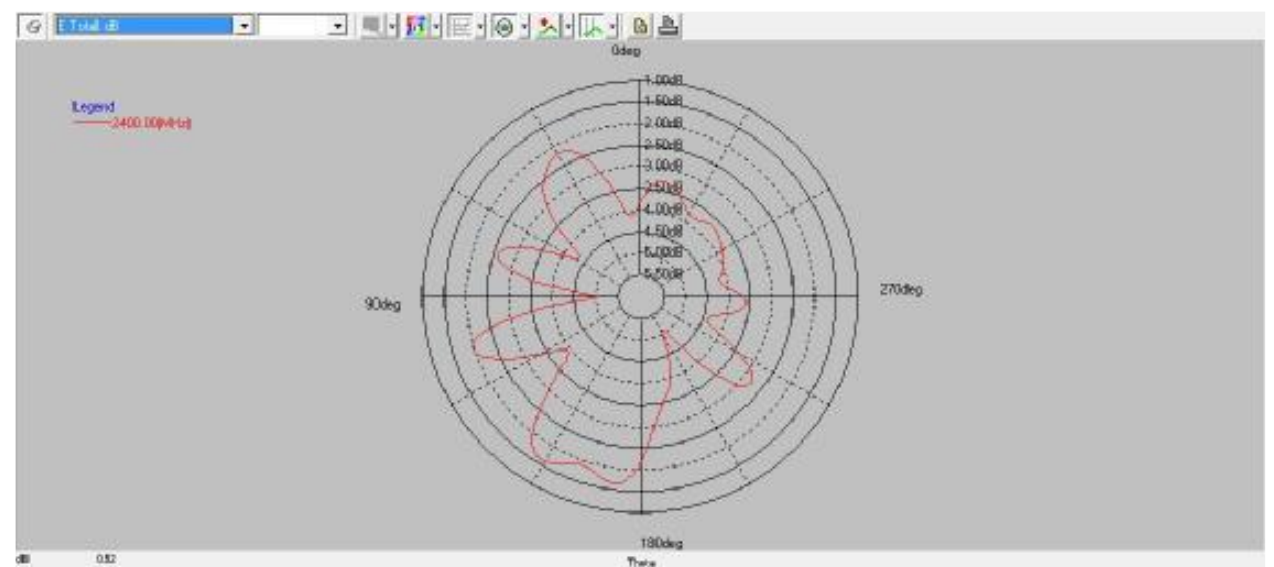
THETA 90
