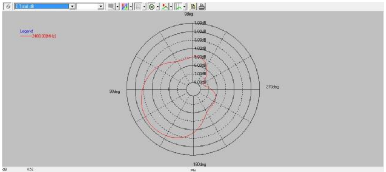
PHI 0
