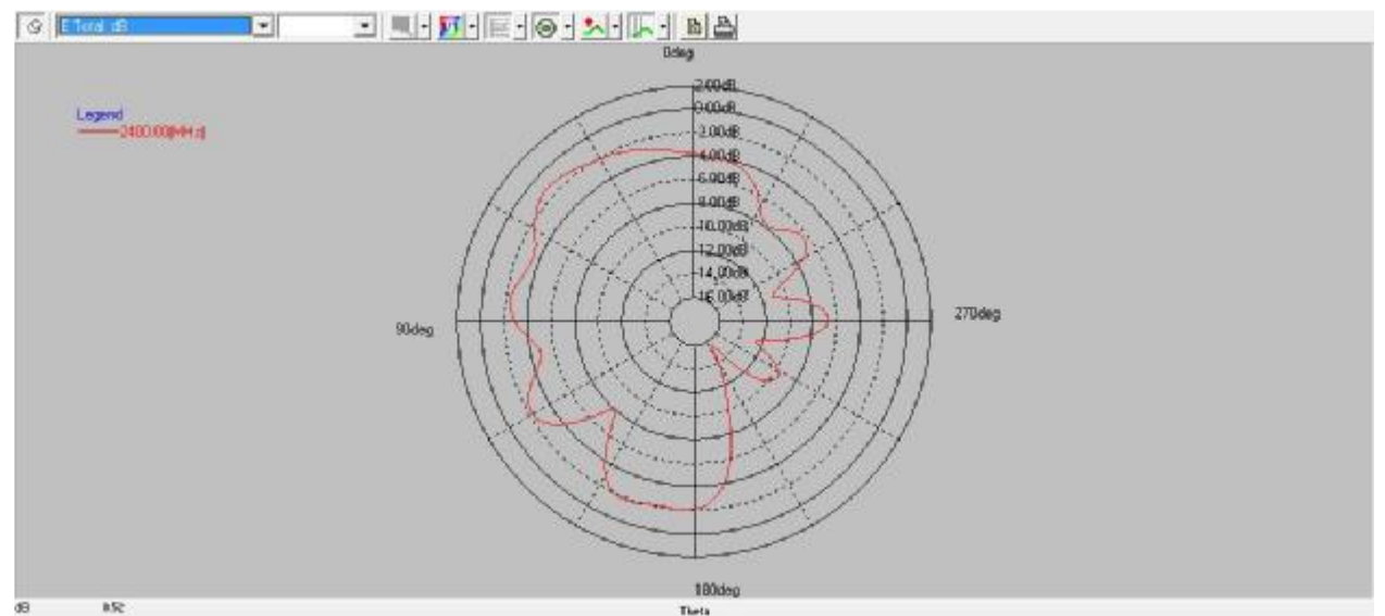
PHI 90
