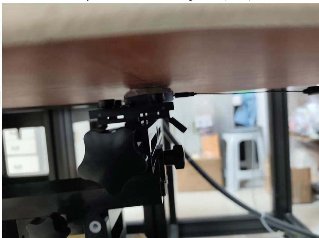
Body Back With Holder Setup Photo (0 mm)
