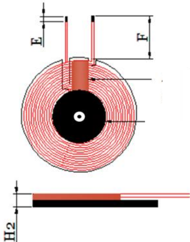
Figure 3: Combination of coil and hard magnetic sheet
