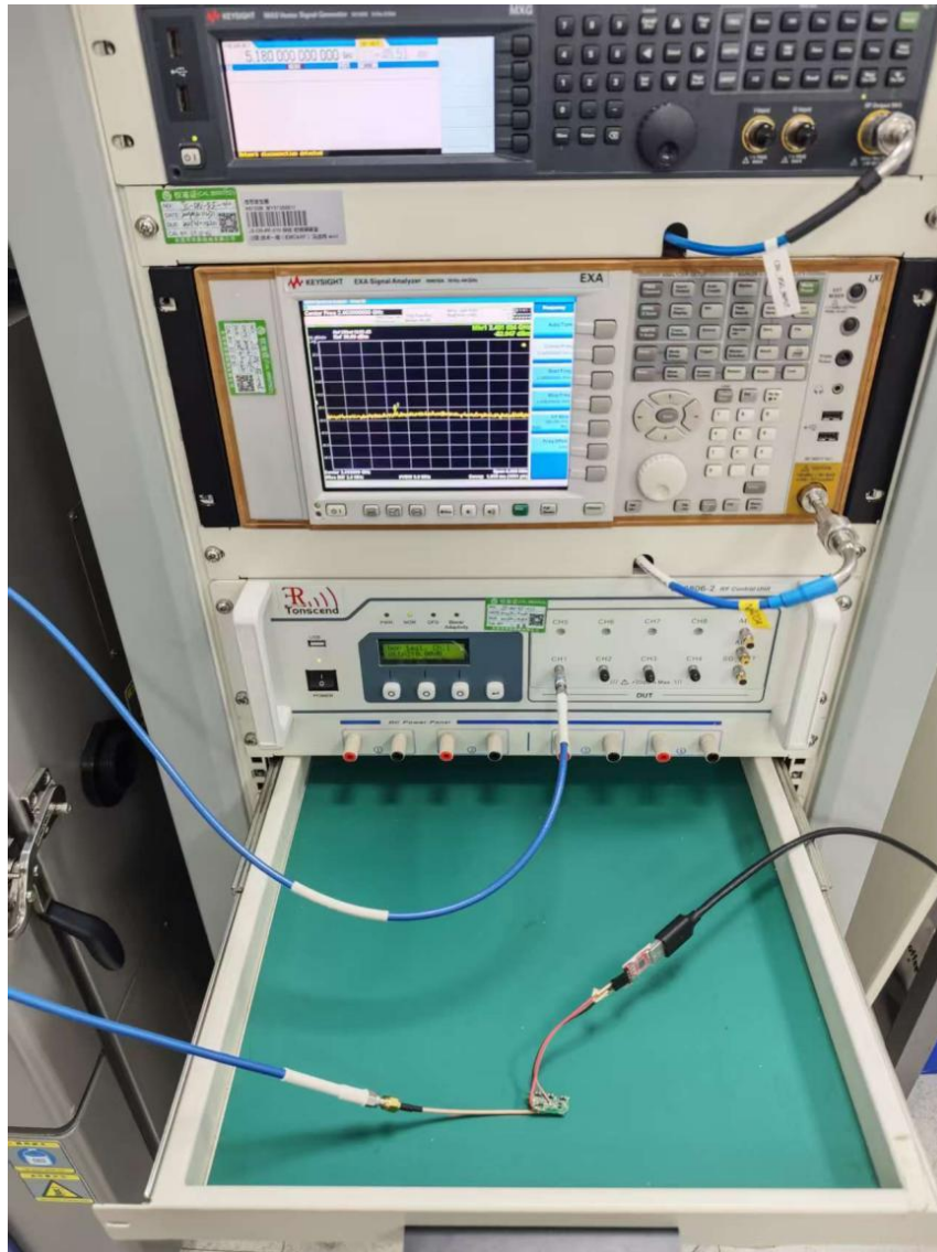
Antenna Terminal Test View
