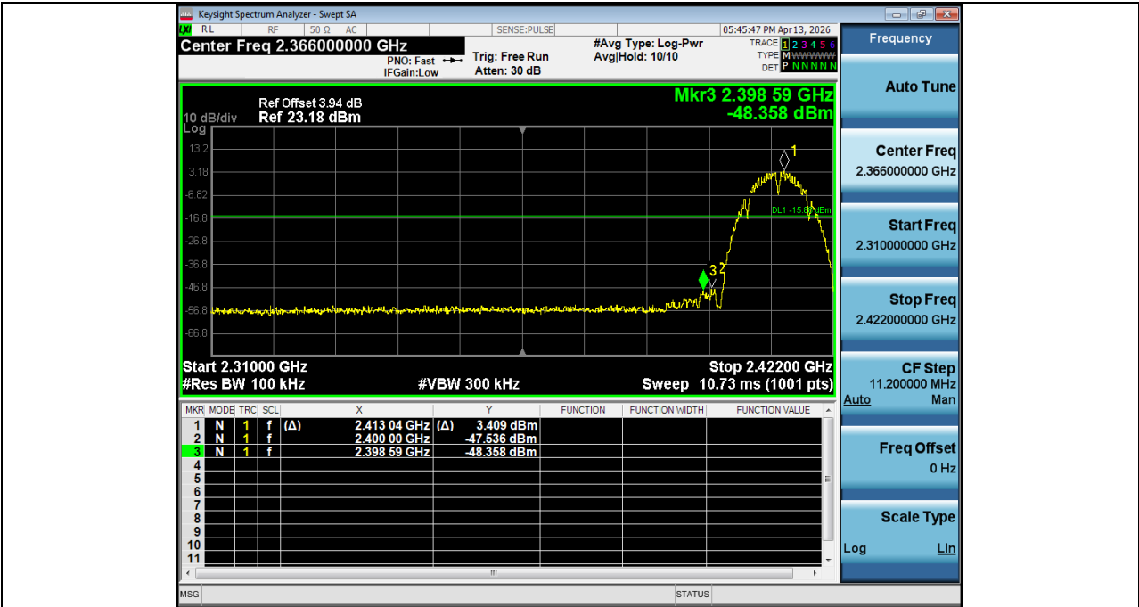
2. Bandedge NVNT_ANT2_802_11b_2412
