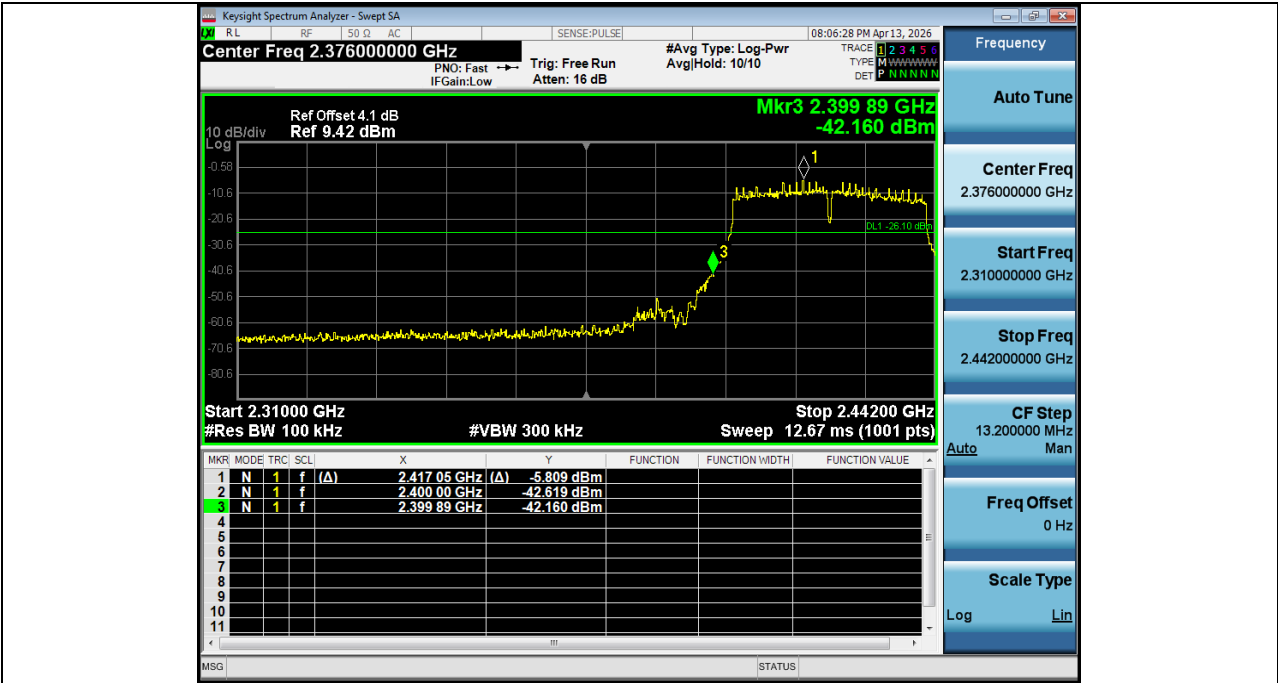
2. Bandedge NVNT_ANT2_802_11n(HT40)_2422
