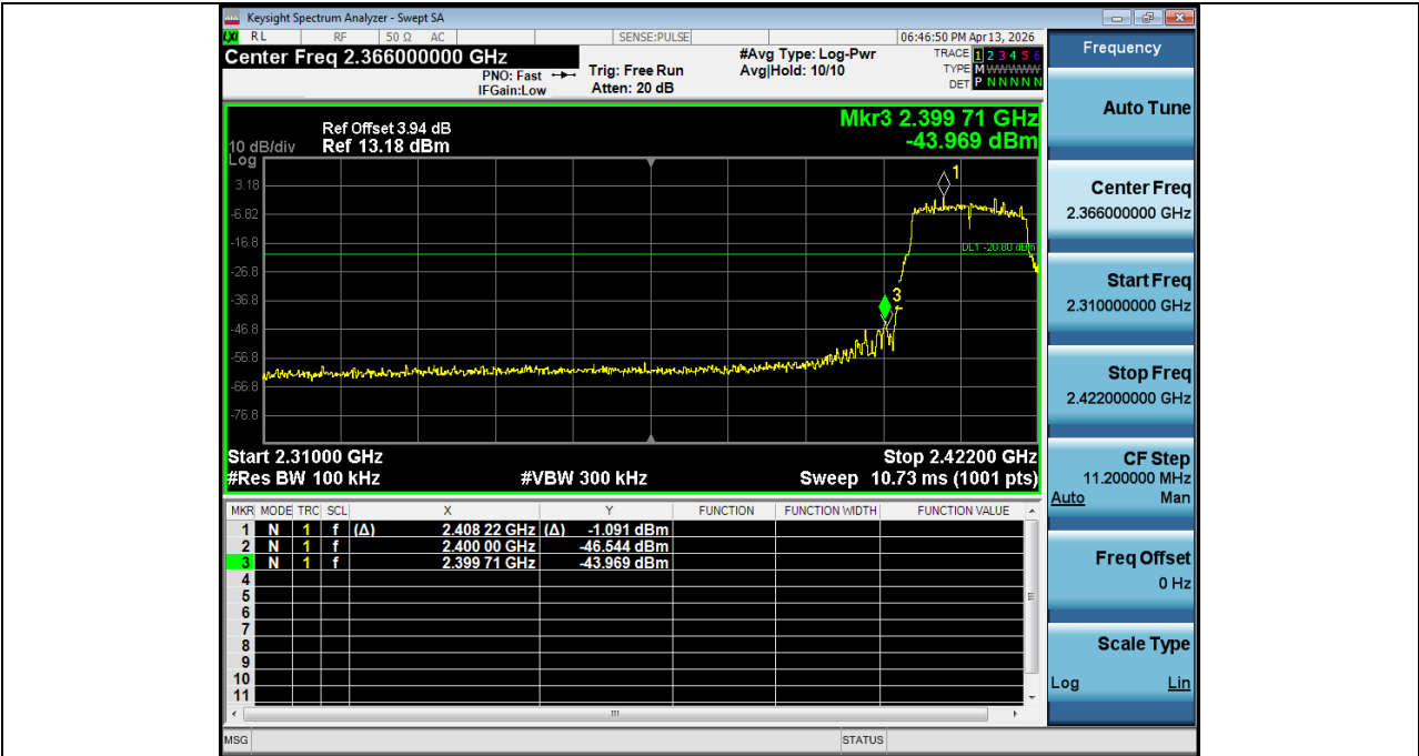
2. Bandedge NVNT_ANT2_802_11g_2412
