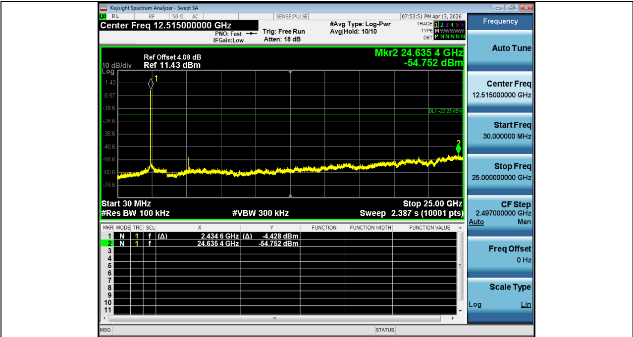
2. Spurious Emission NVNT_ANT2_802_11n(HT20)_2437
