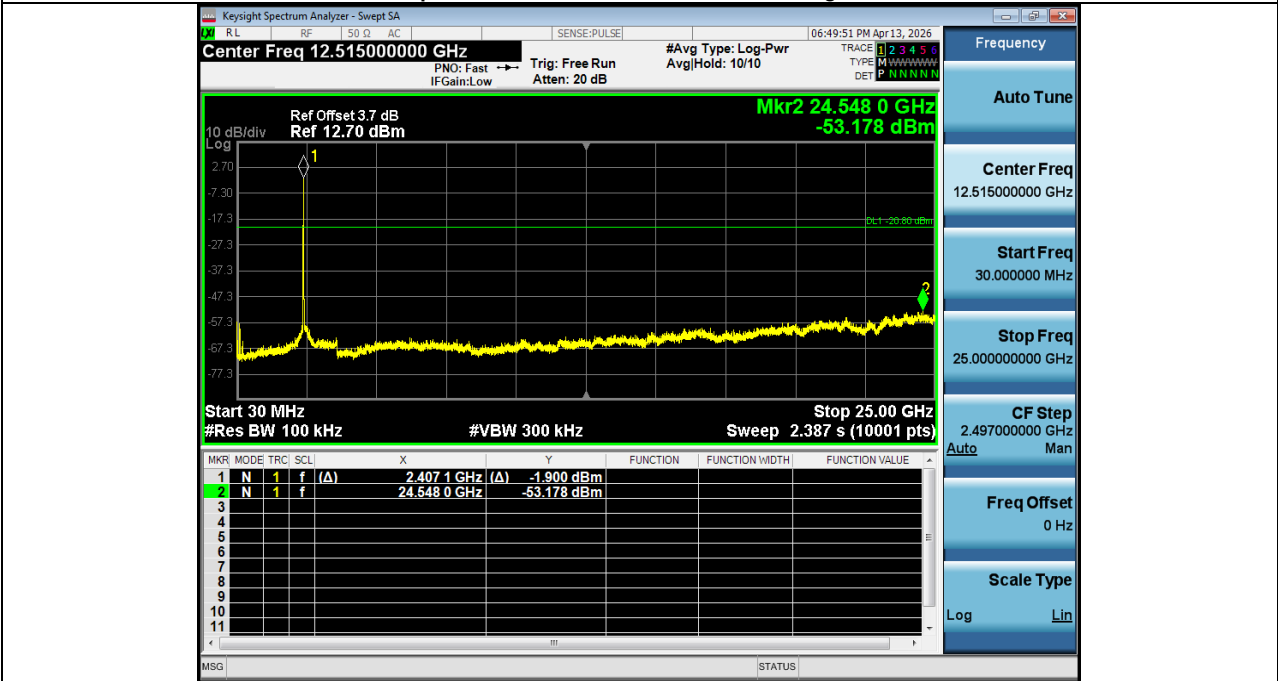
2. Spurious Emission NVNT_ANT2_802_11g_2412
