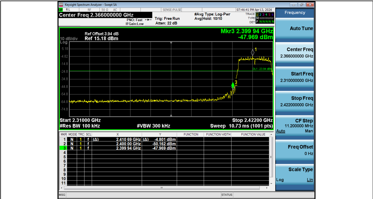
2. Bandedge NVNT_ANT2_802_11n(HT20)_2412
