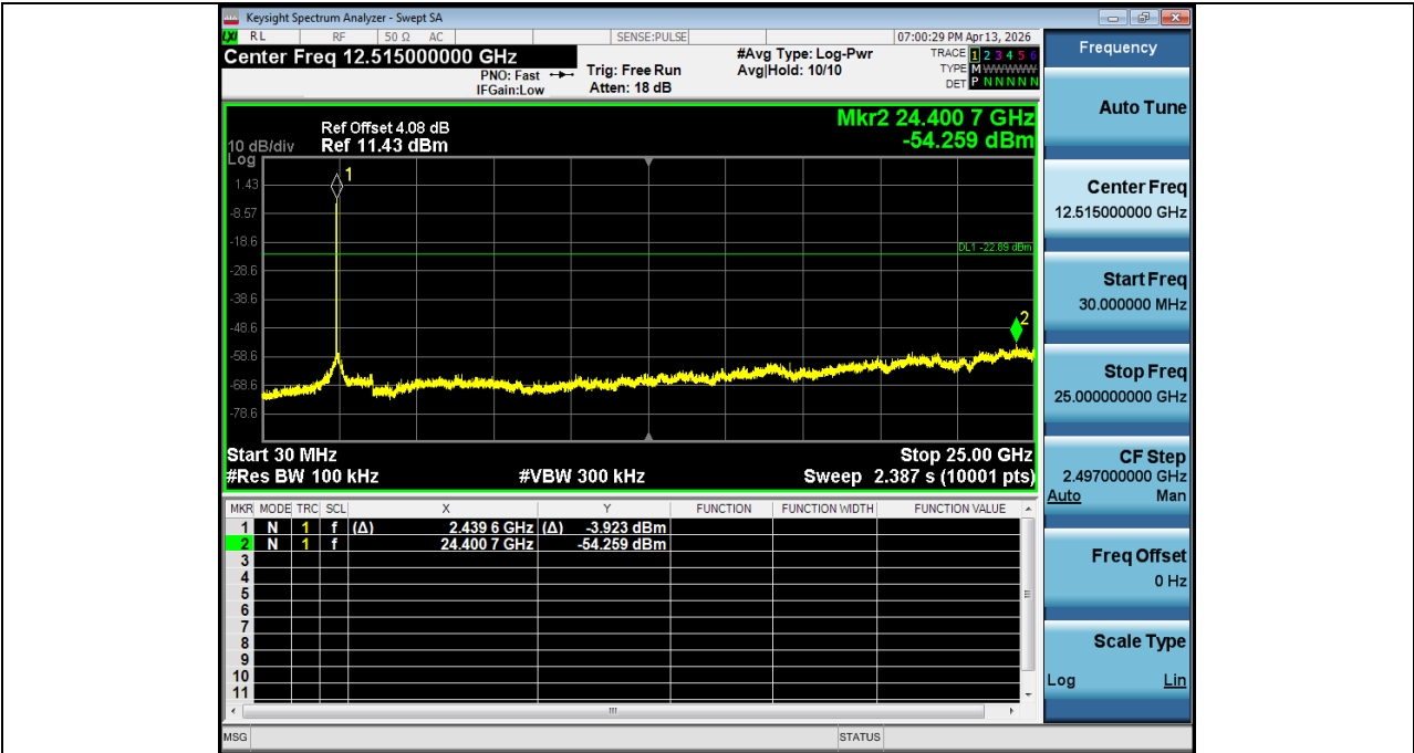
2. Spurious Emission NVNT_ANT2_802_11g_2437
