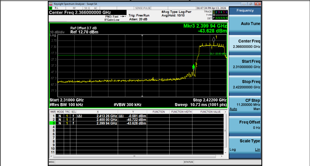
2. Bandedge NVNT_ANT2_802_11g_2412
