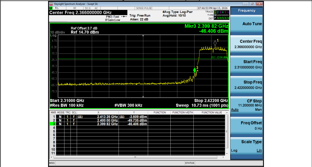
2. Bandedge NVNT_ANT2_802_11n(HT20)_2412
