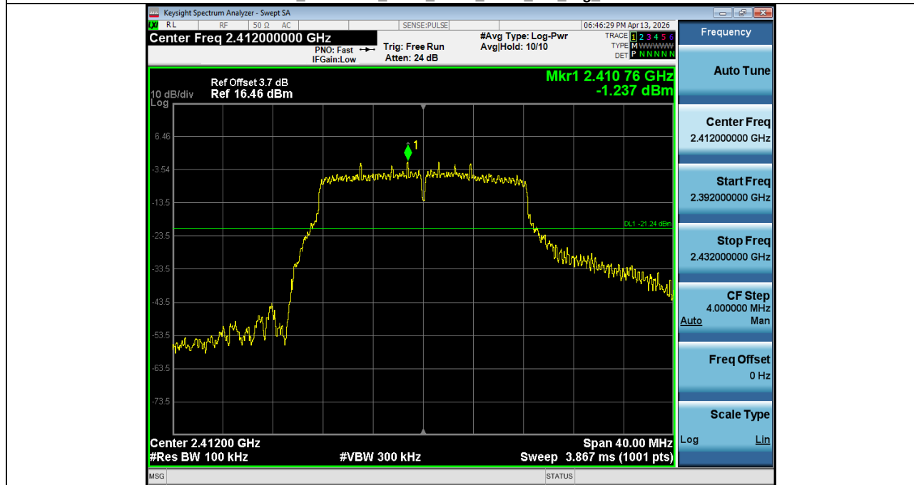
2. Bandedge_NVNT_ANT1_802_11g_2412
