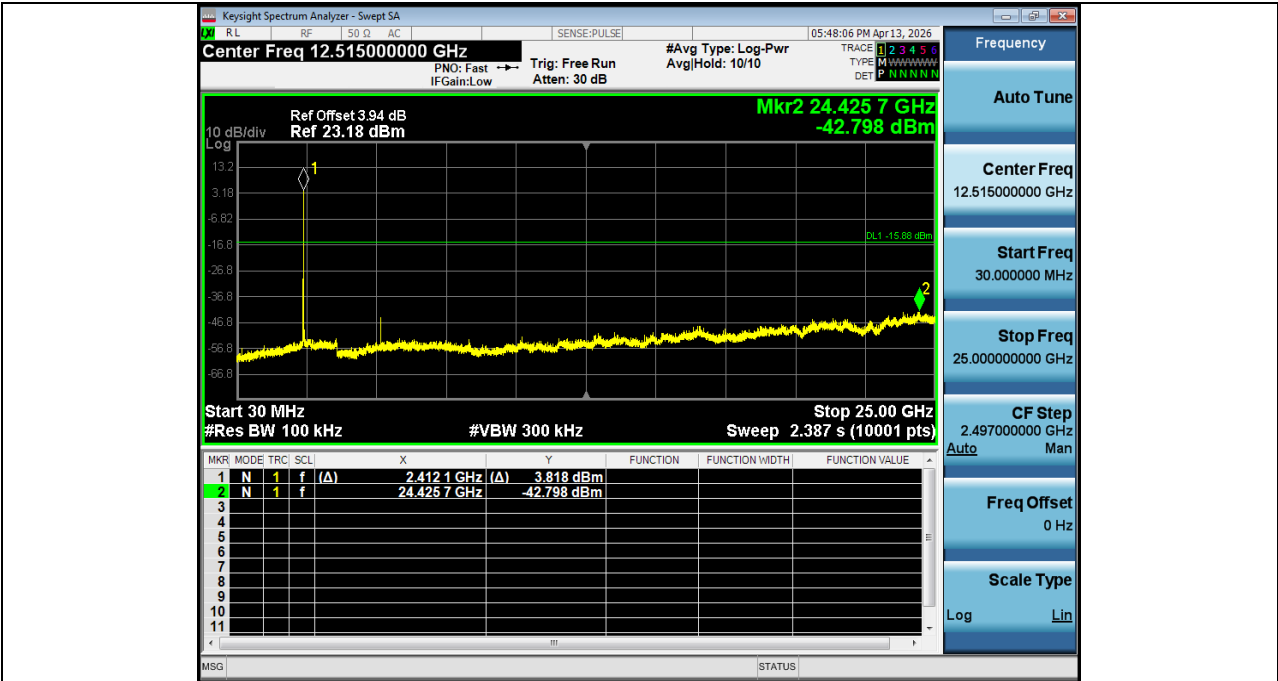
2. Spurious Emission NVNT_ANT2_802_11b_2412
