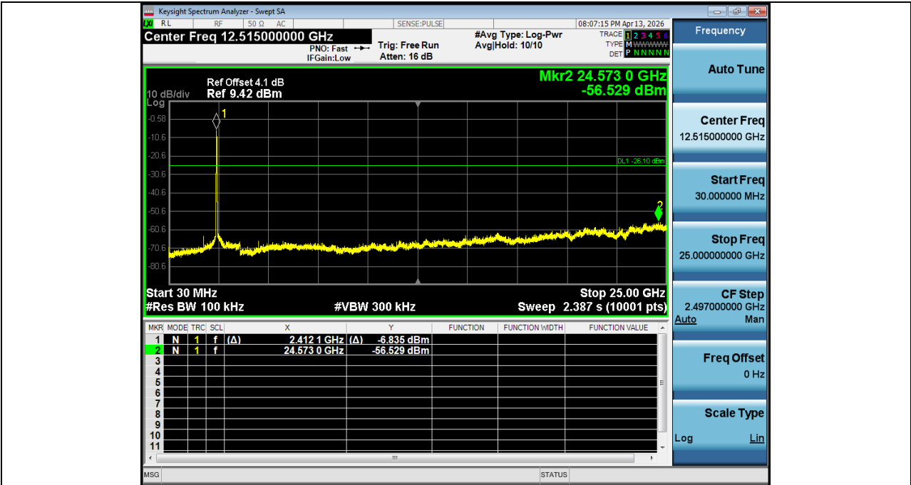
2. Spurious Emission NVNT_ANT2_802_11n(HT40)_2422
