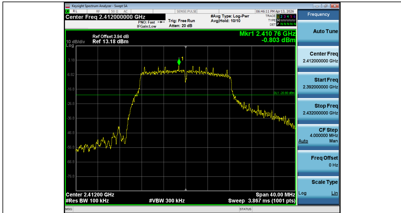
1. Reference Level NVNT_ANT2_802_11g_2412
