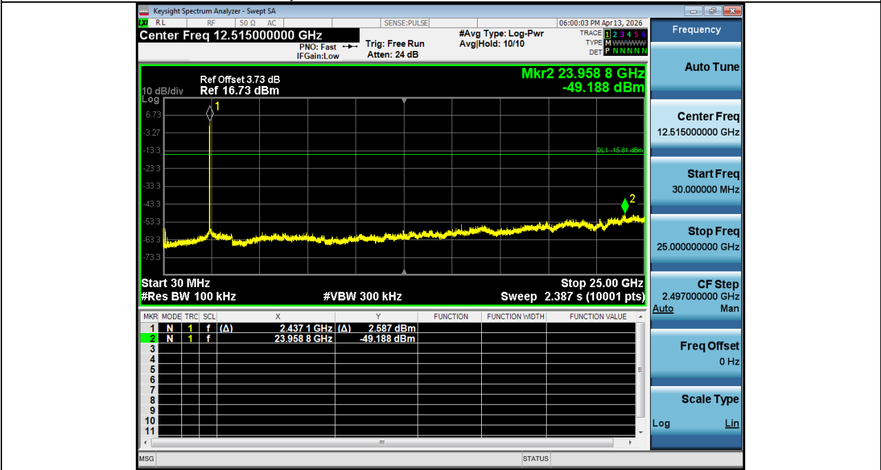
2. Spurious Emission NVNT_ANT2_802_11b_2437
