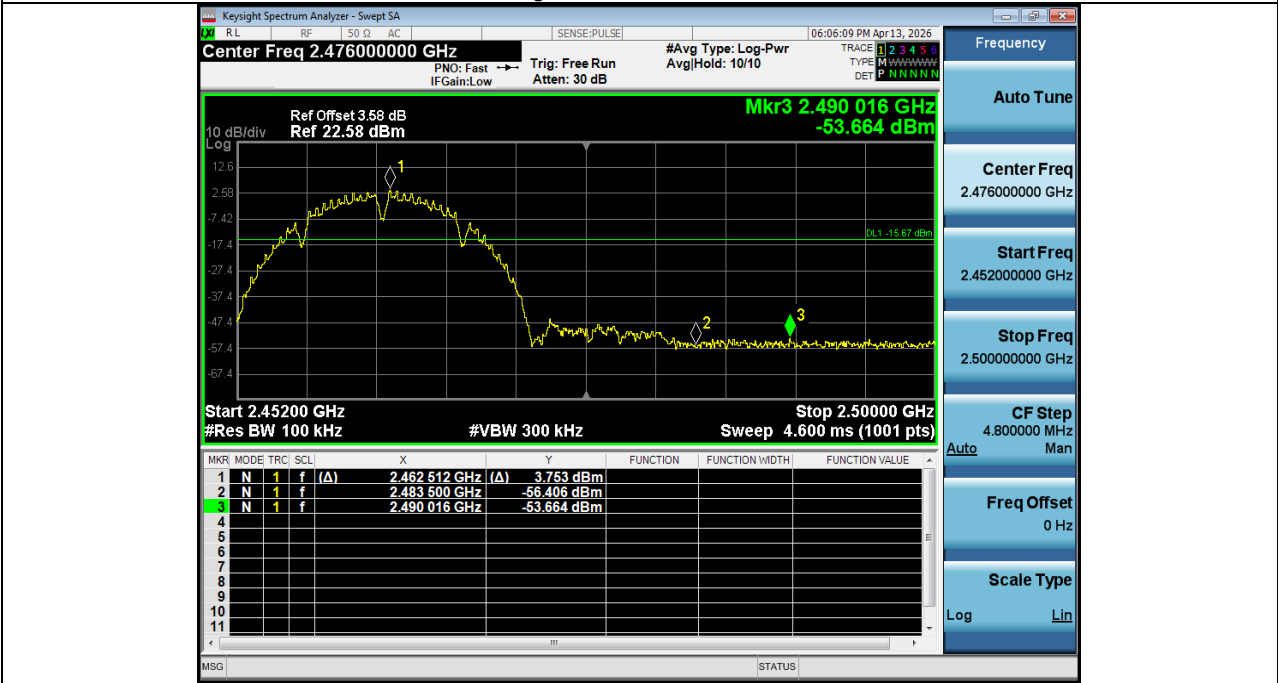
2. Bandedge NVNT_ANT2_802_11b_2462
