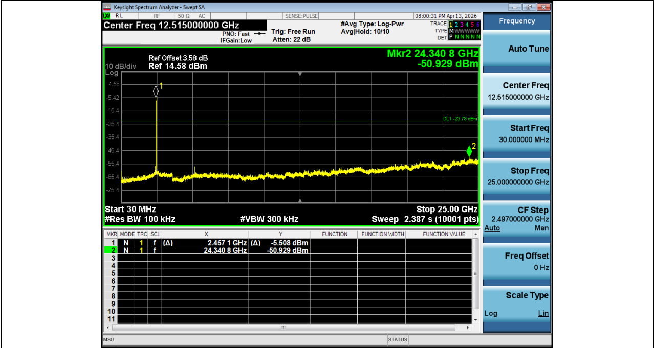
2. Spurious Emission NVNT_ANT2_802_11n(HT20)_2462
