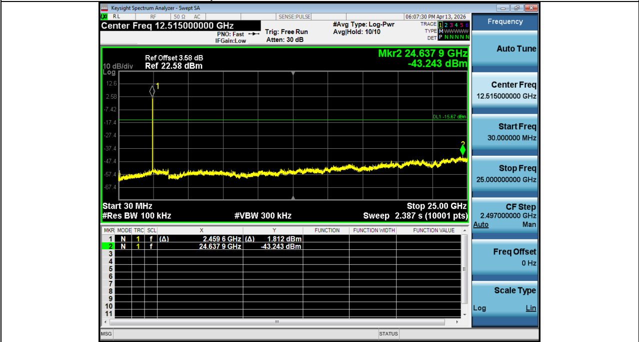
2. Spurious Emission NVNT_ANT2_802_11b_2462
