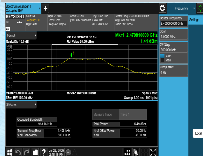
TX-Ant3-2480-PASS
