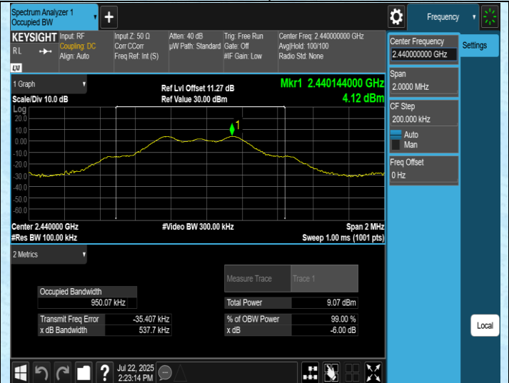
TX-Ant4-2440-PASS
