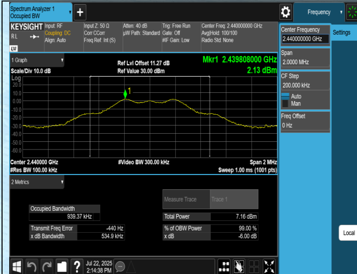
TX-Ant3-2440-PASS
