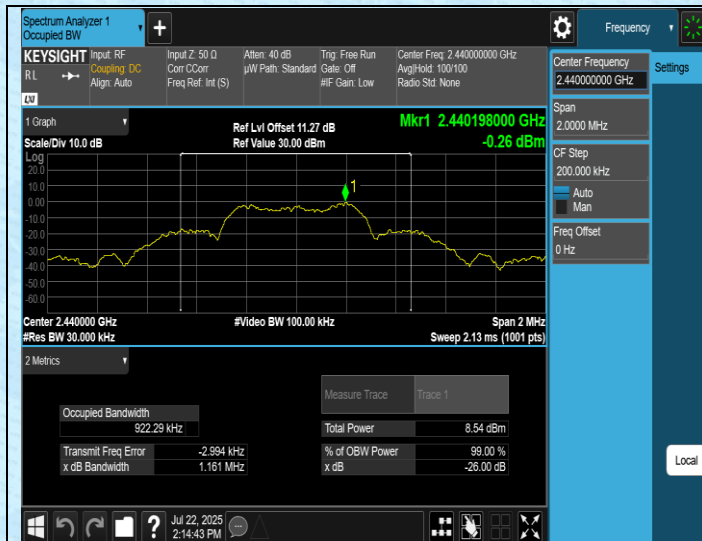
TX-Ant3-2440
