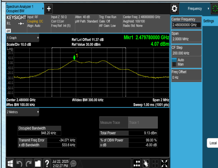
TX-Ant1-2480-PASS
