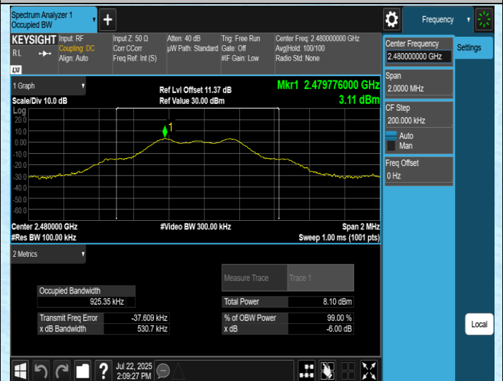
TX-Ant2-2480-PASS
