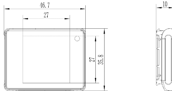
Figure 2-3 1.54" dimension
