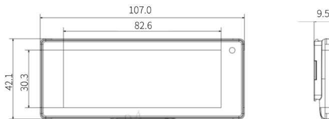
Figure 2-8 3.46" dimension
