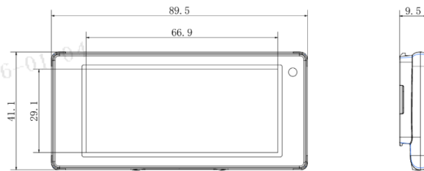
Figure 2-7 2.9" dimension
