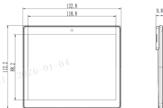
Figure 2-11 4.37" dimension
