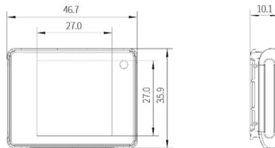
Figure 2-3 1.54" dimension
