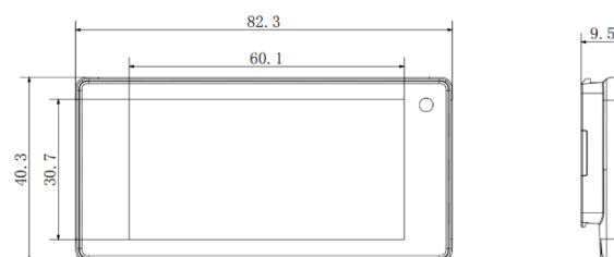
Figure 2-5 2.13" dimension
