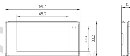
Figure 2-5 2.13" dimension
