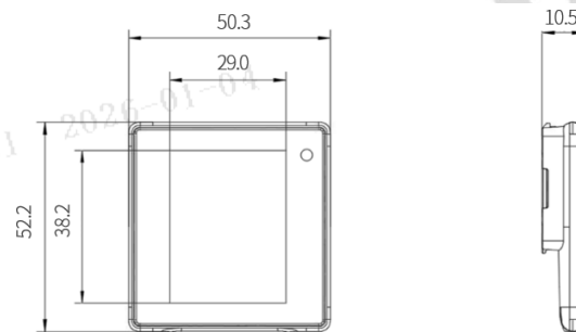
Figure 2-4 2.0" dimension
