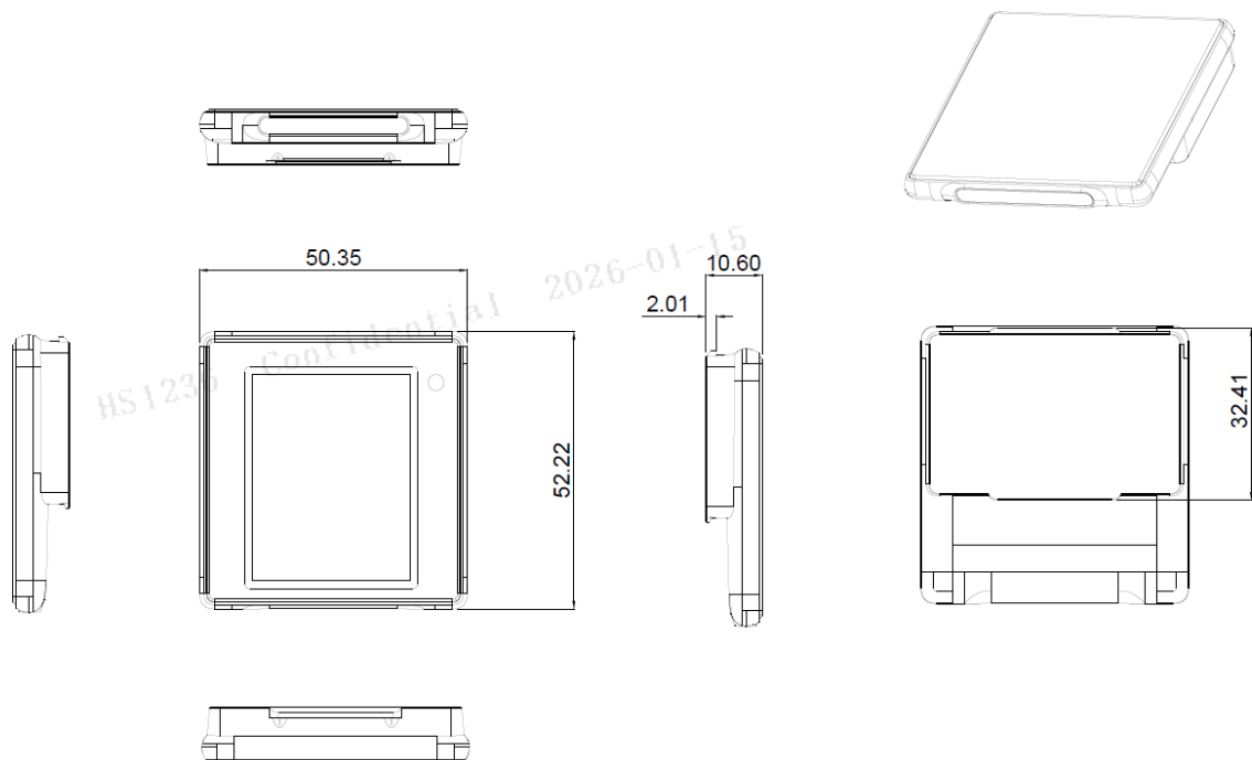
Figure 2-4 2.0" dimension
