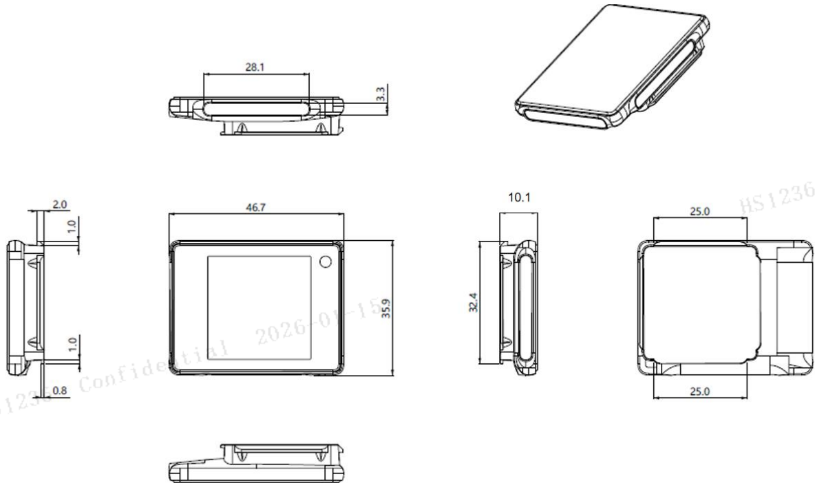
Figure 2-3 1.54" dimension
