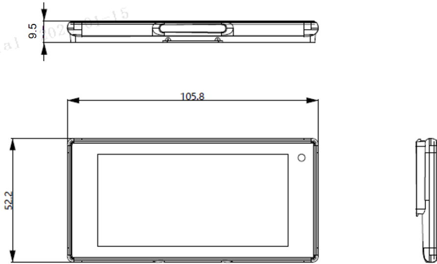
Figure 2-9 3.5" dimension
