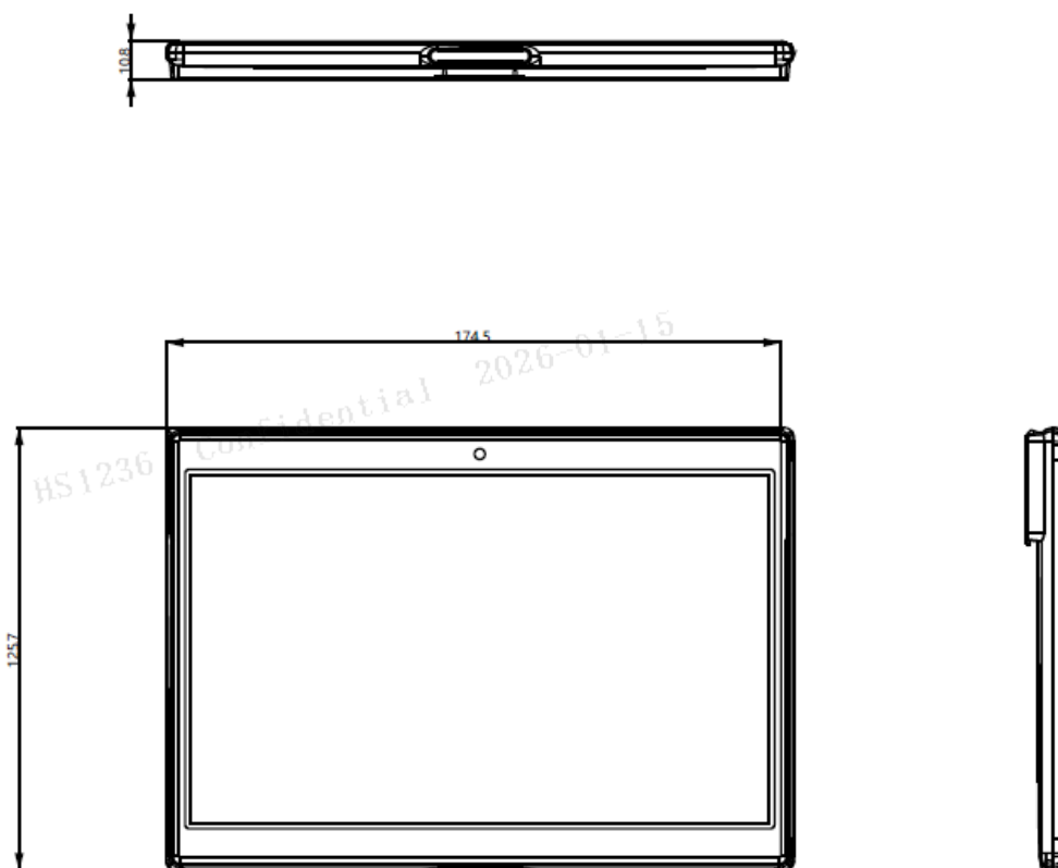
Figure 2-12 7.5" dimension
