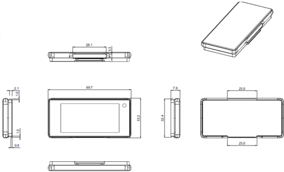
Figure 2-3 2.30" dimension
