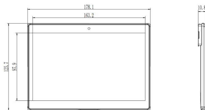
Figure 2-12 7.5" dimension
