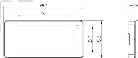
Figure 2-5 2.13" dimension
