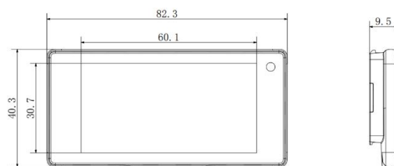
Figure 2-6 2.66" dimension
