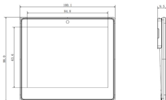
Figure 2-10 4.2" dimension
