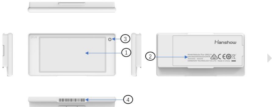
Figure 2-2 and Table 2-1.
