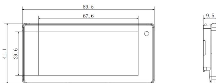
Figure 2-6 2.66" dimension
