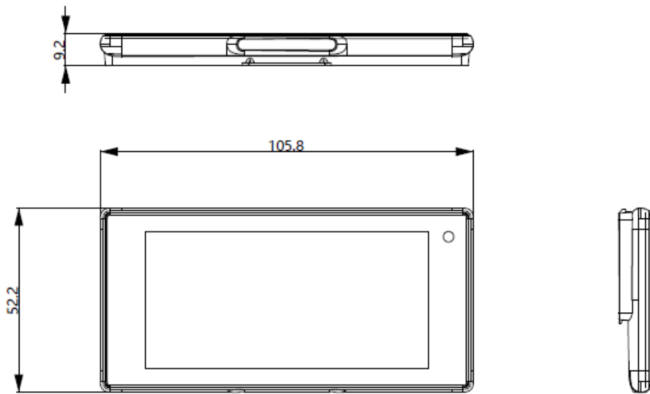
Figure 2-93.5" dimension
