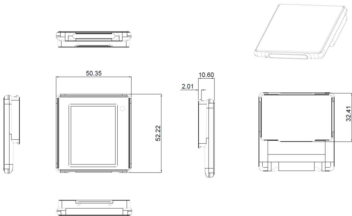
Figure 2-42.0" dimension
