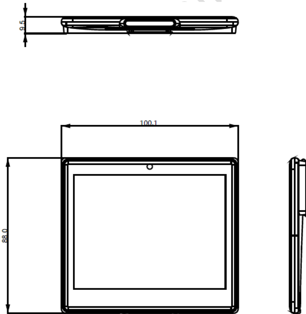
Figure 2-10 4.2" dimension
