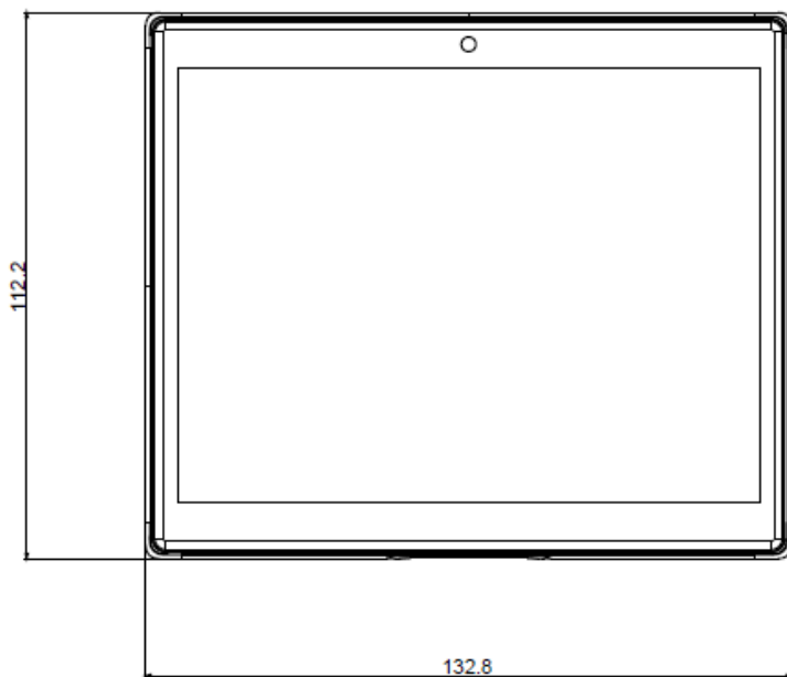
Figure 2-111 5.83" dimension
