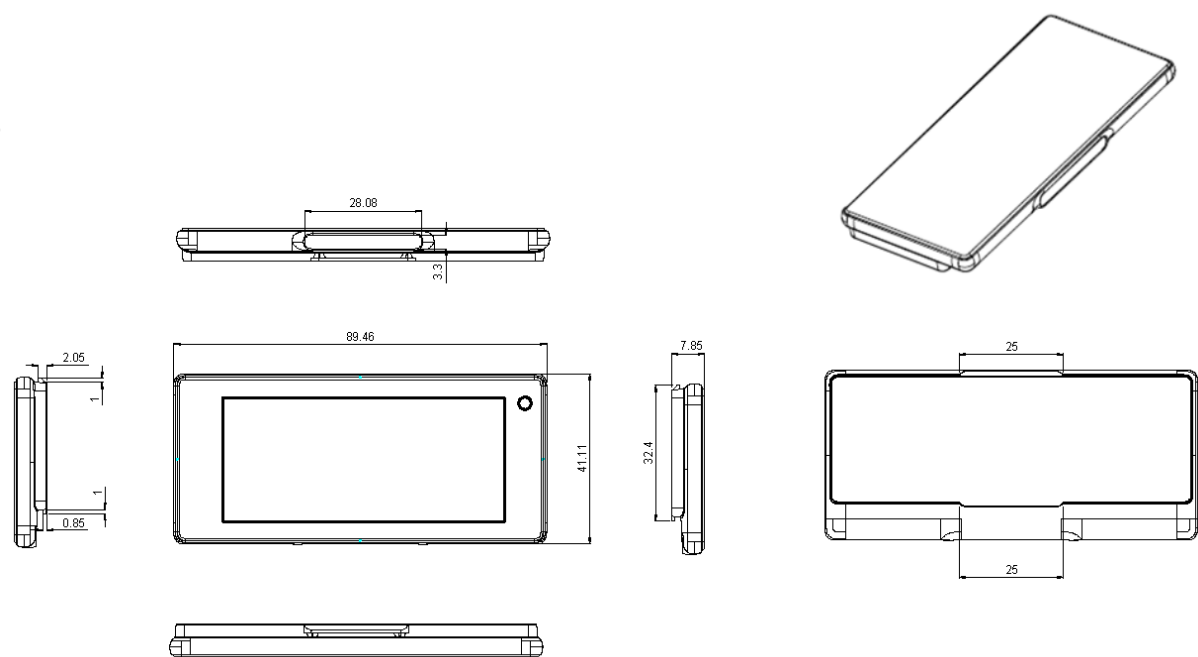
Figure 2-72.9" dimension
