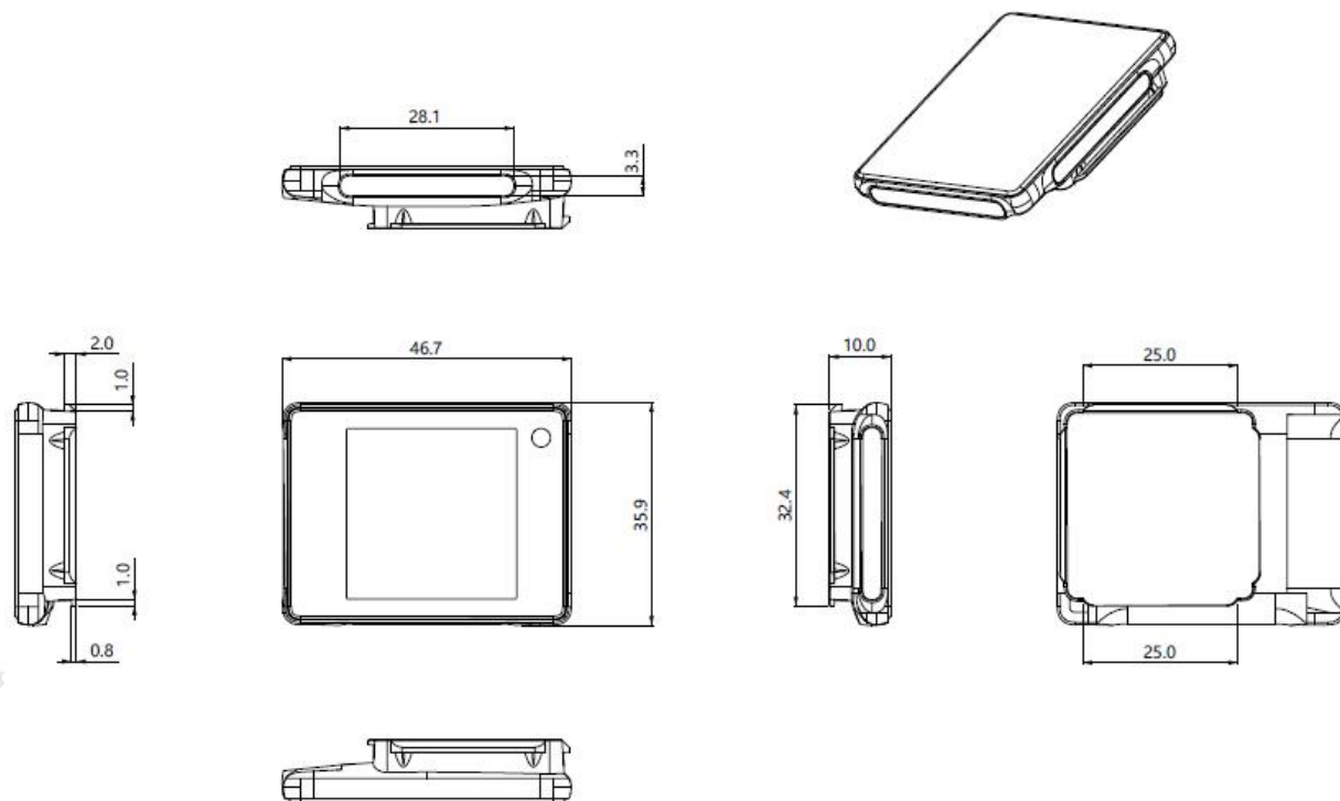
Figure 2-3 1.54" dimension
