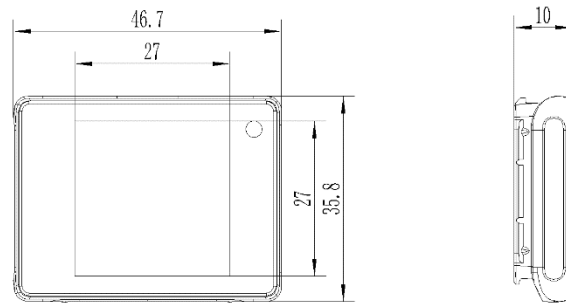
Figure 2-3 1.54" dimension
