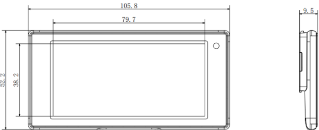
Figure 2-9 3.5" dimension
