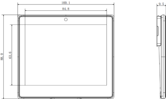
Figure 2-10 4.2" dimension
