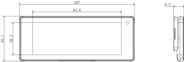
Figure 2-8 3.46" dimension
