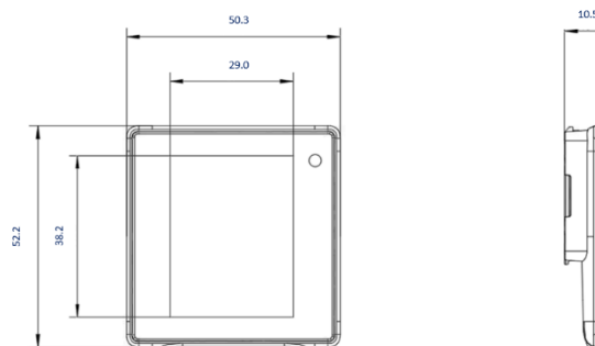
Figure 2-4 2.0" dimension
