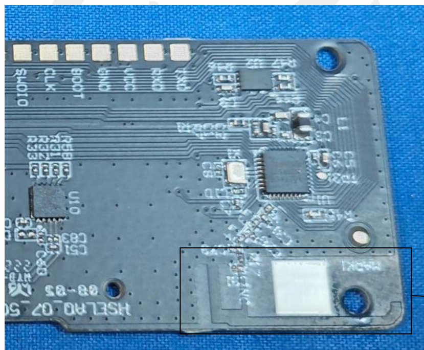
PCB antenna
