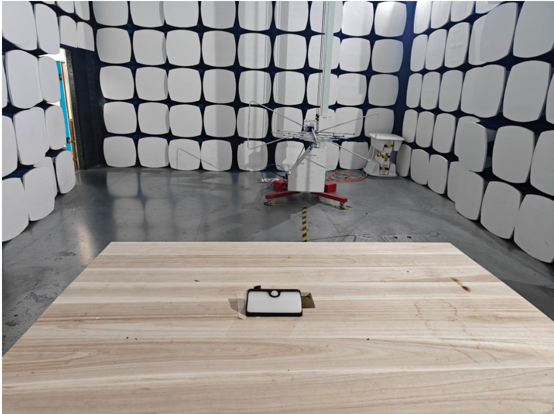
Radiated Emission (30MHz-1GHz)
