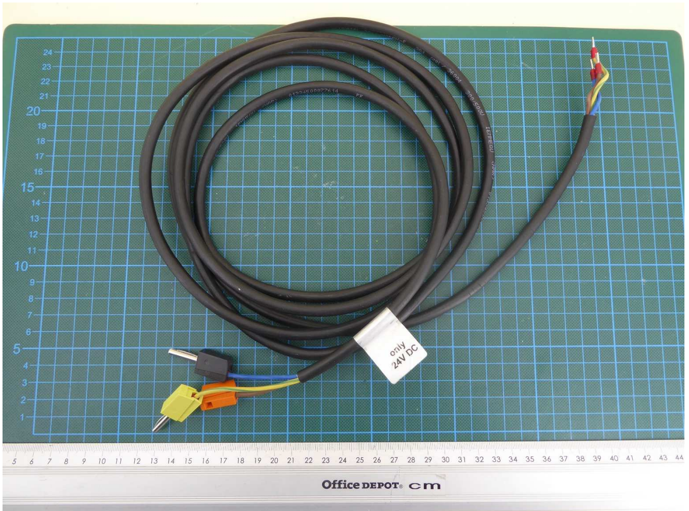
Power supply line – 24V DC
