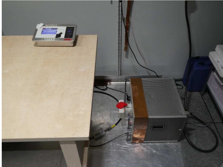
Test setup AC powerline conducted EUT1 (120V/230V AC)
