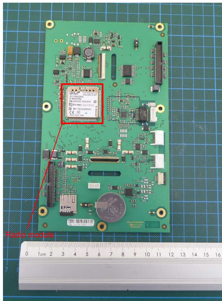
PCB 6 – top view
