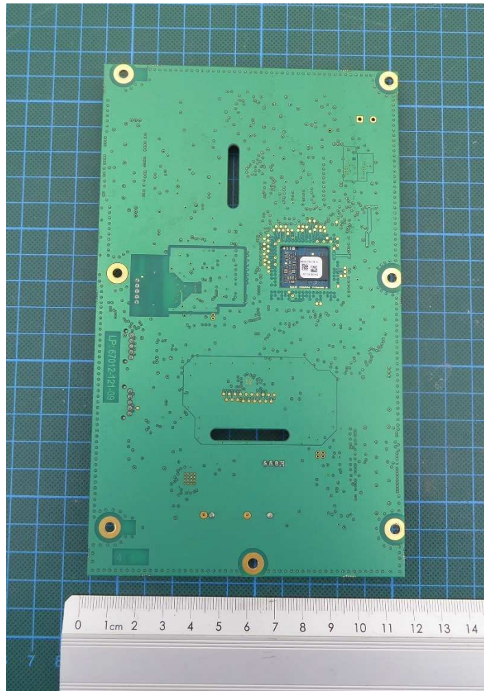
PCB 6 – bottom view
