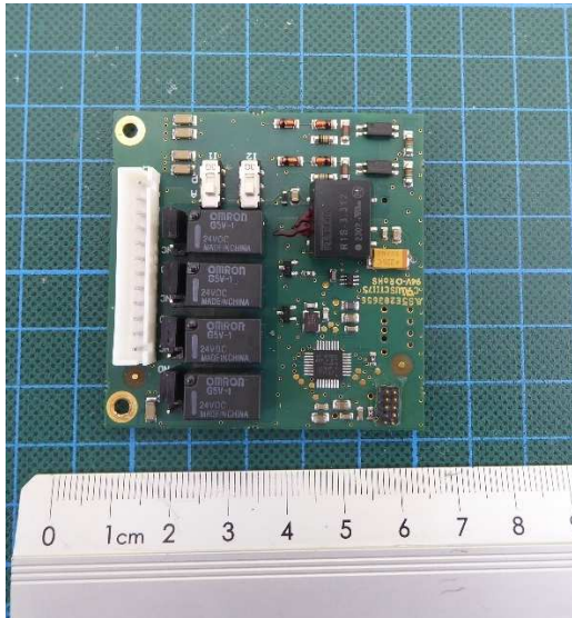
PCB 2 – top view
