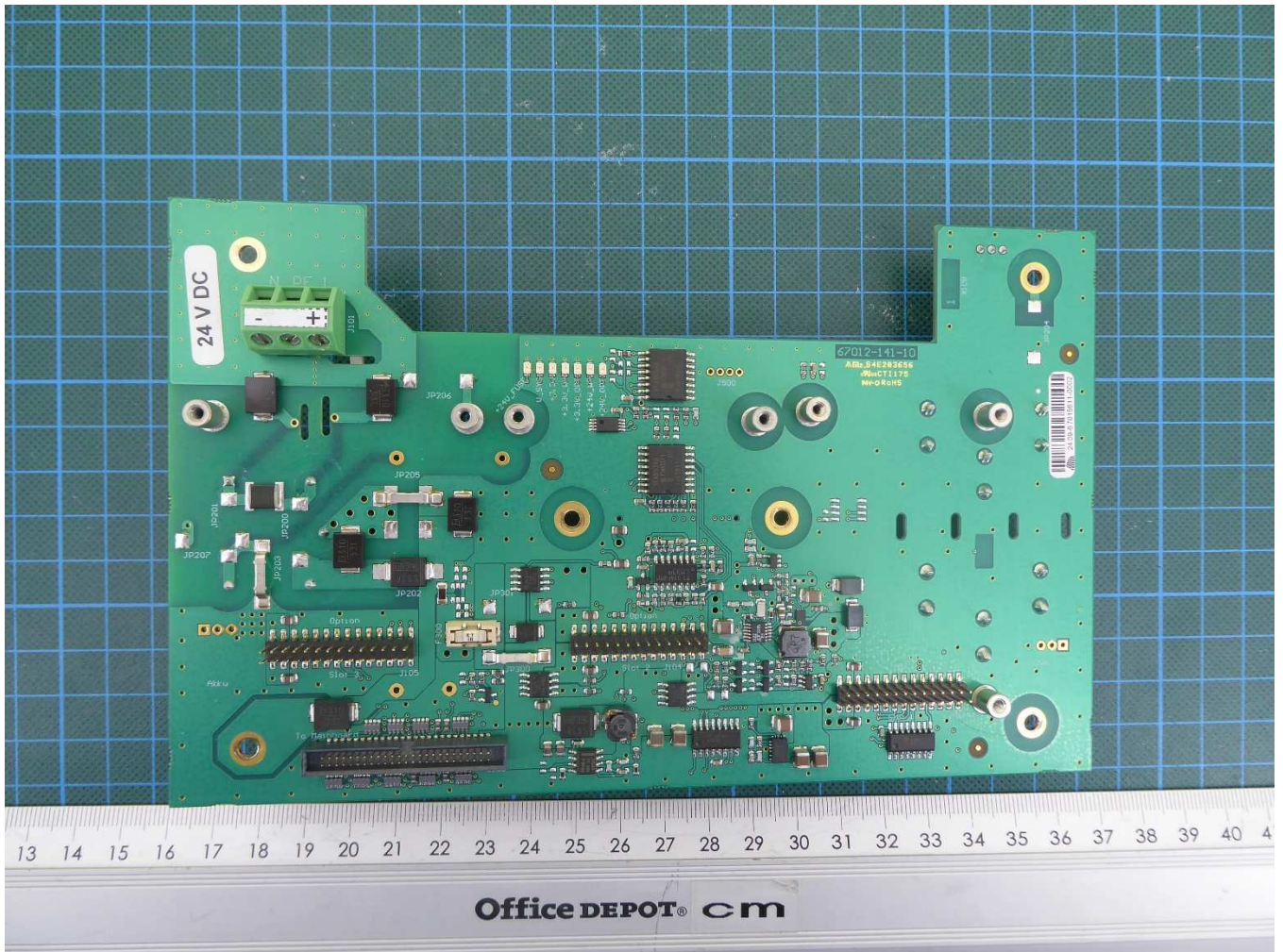
PCB 1 (connection board) - top view
