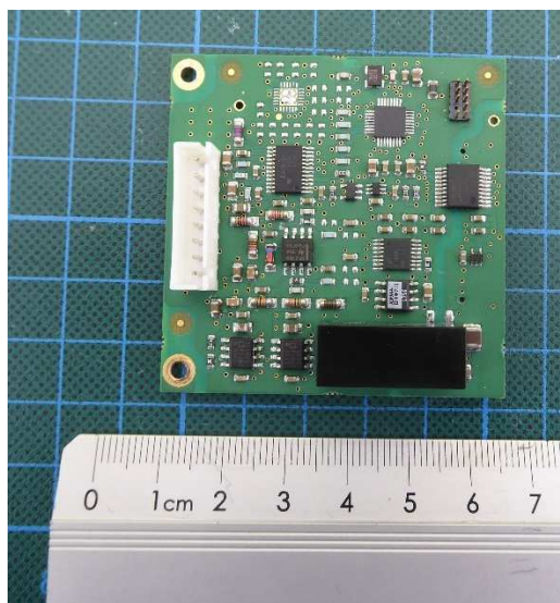
PCB 3 – top view
