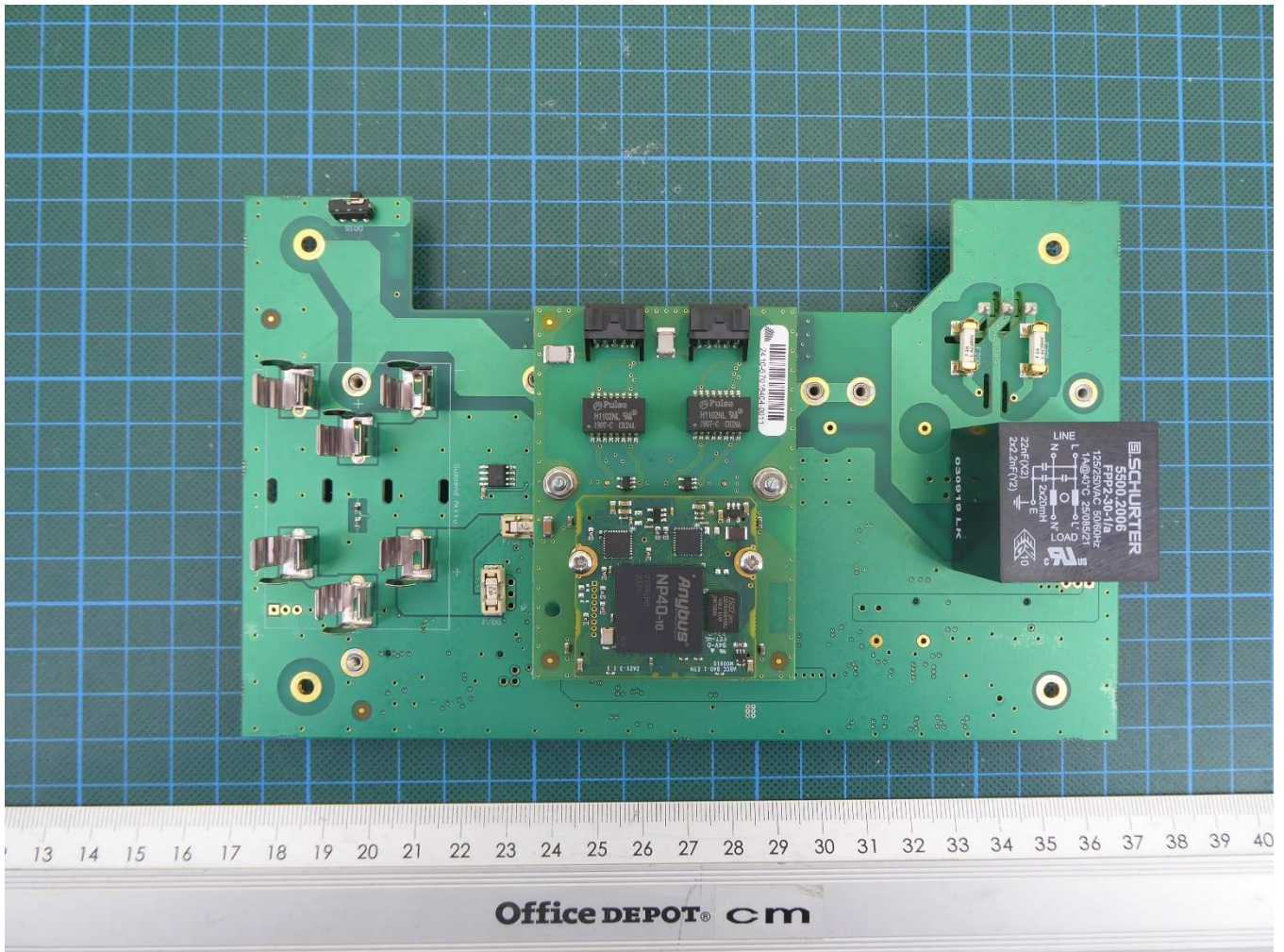
PCB 1 (connection board) - bottom view
