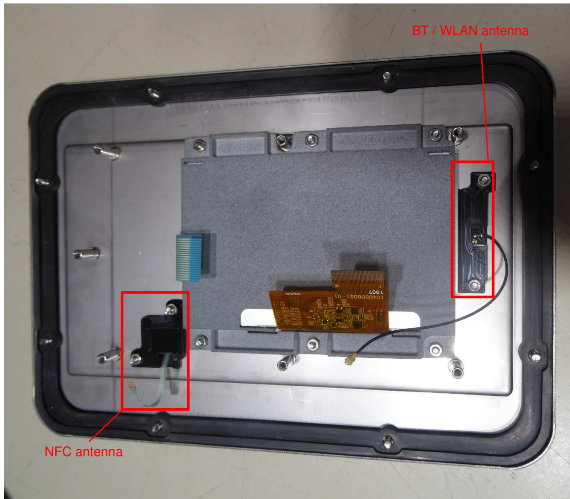
EUT – display plate
