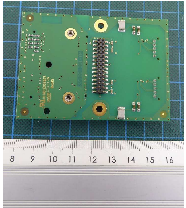
PCB 5 – bottom view
