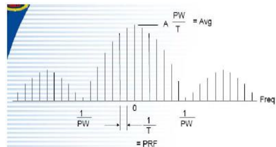
Frequency Spectrum of Periodic Square Pulse
