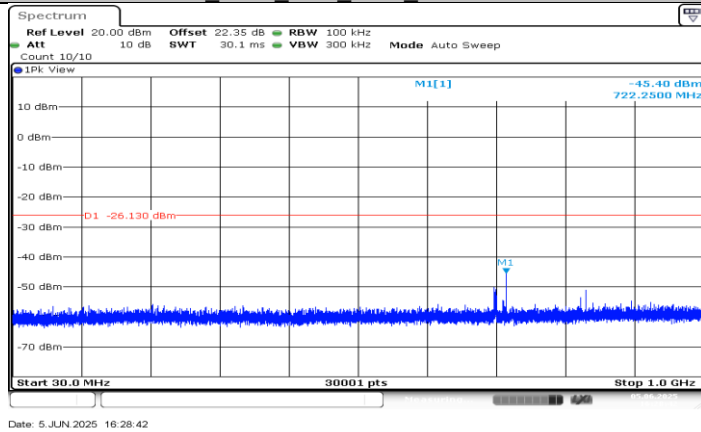
BLE_125K Ant1_2480_30~1000
