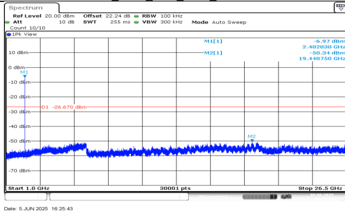
BLE_125K Ant1_2402_1000~26500
