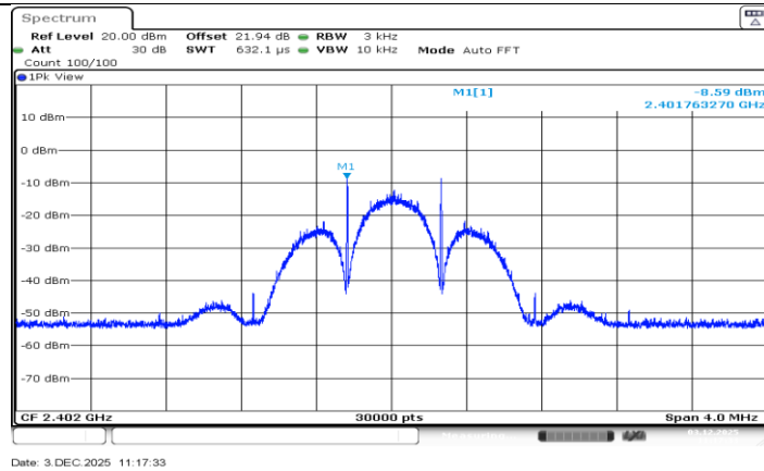
BLE_125K_Ant1_2402
