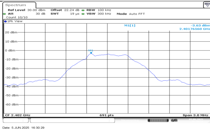
BLE_500K Ant1_2402_0~Reference
