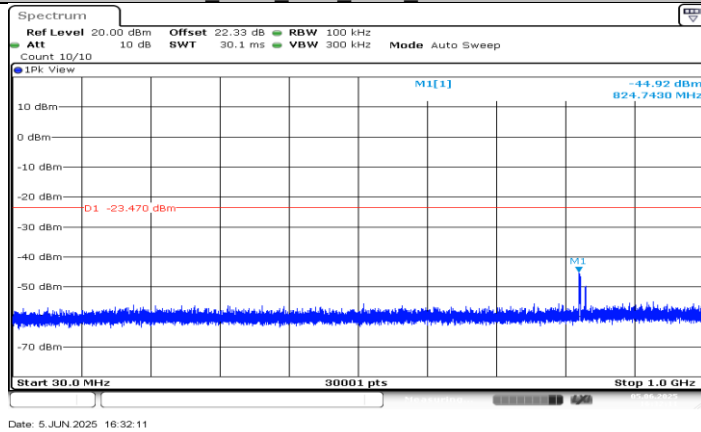
BLE_500K Ant1_2440_30~1000
