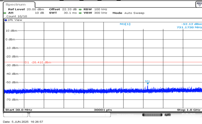
BLE_125K Ant1_2440_30~1000
