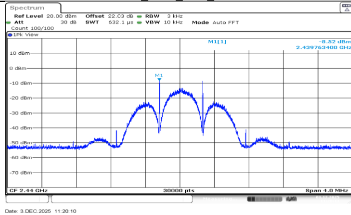
BLE_125K_Ant1_2440
