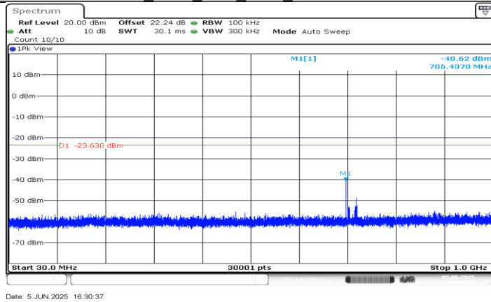
BLE_500K Ant1_2402_30~1000
