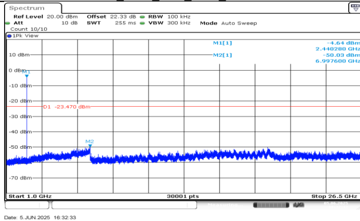
BLE_500K Ant1_2440_1000~26500
