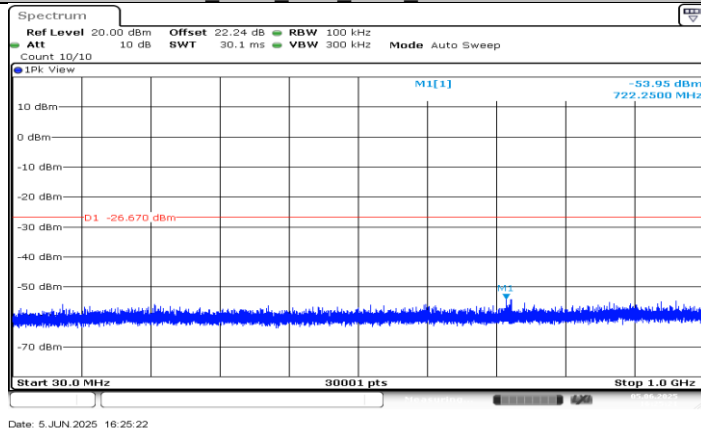
BLE_125K Ant1_2402_30~1000
