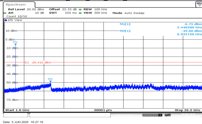
BLE_125K Ant1_2440_1000~26500
