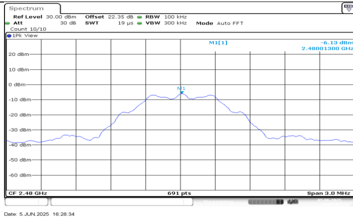
BLE_125K Ant1_2480_0~Reference
