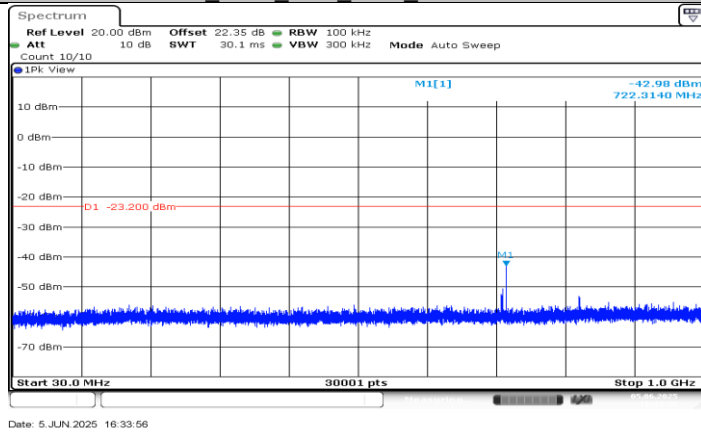
BLE_500K Ant1_2480_30~1000
