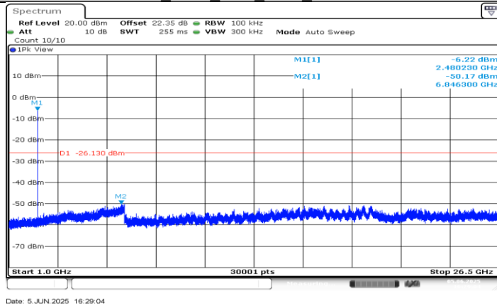
BLE_125K Ant1_2480_1000~26500
