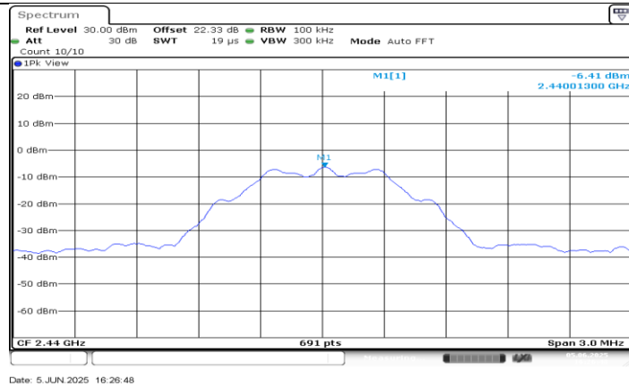
BLE_125K Ant1_2440_0~Reference
