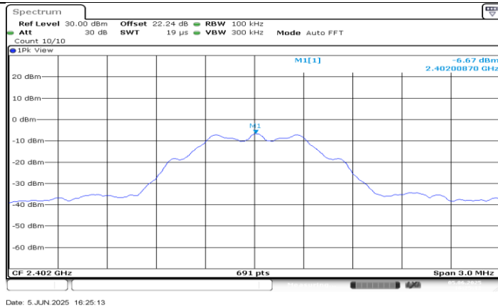
BLE_125K Ant1_2402_0~Reference
