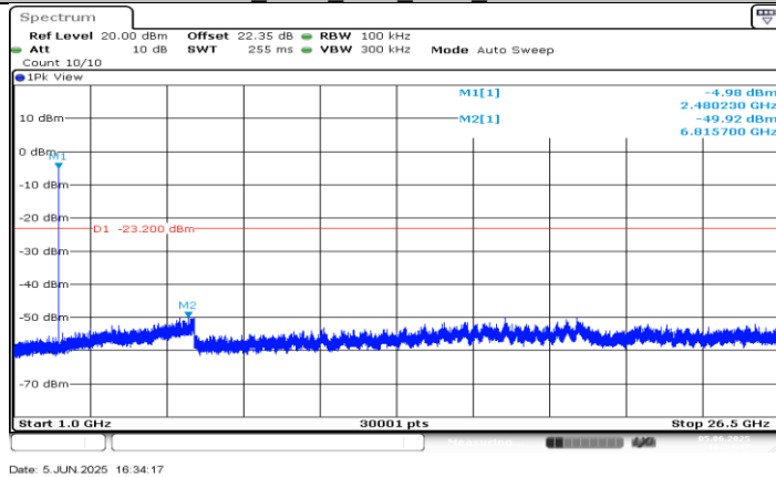
BLE_500K Ant1_2480_1000~26500
