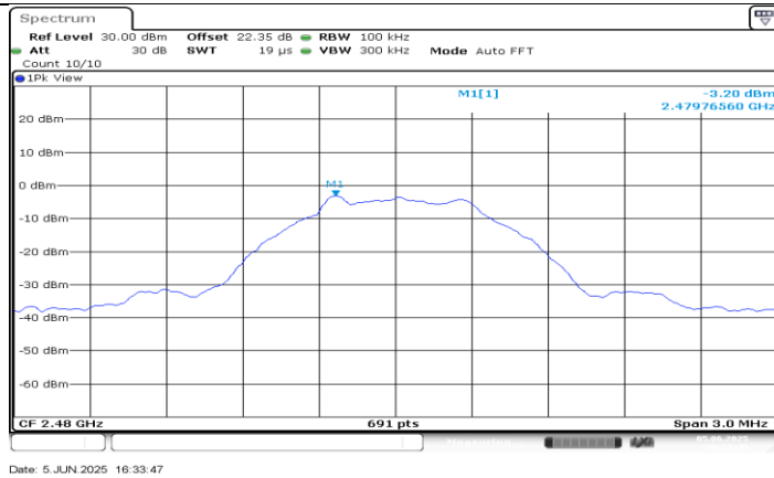
BLE_500K Ant1_2480_0~Reference
