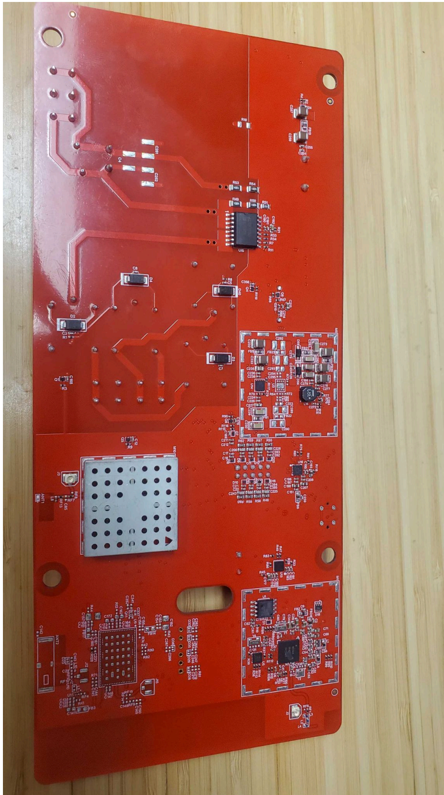
Figure 2: Big Dipper PCB-4 Board Bottom With Shield
