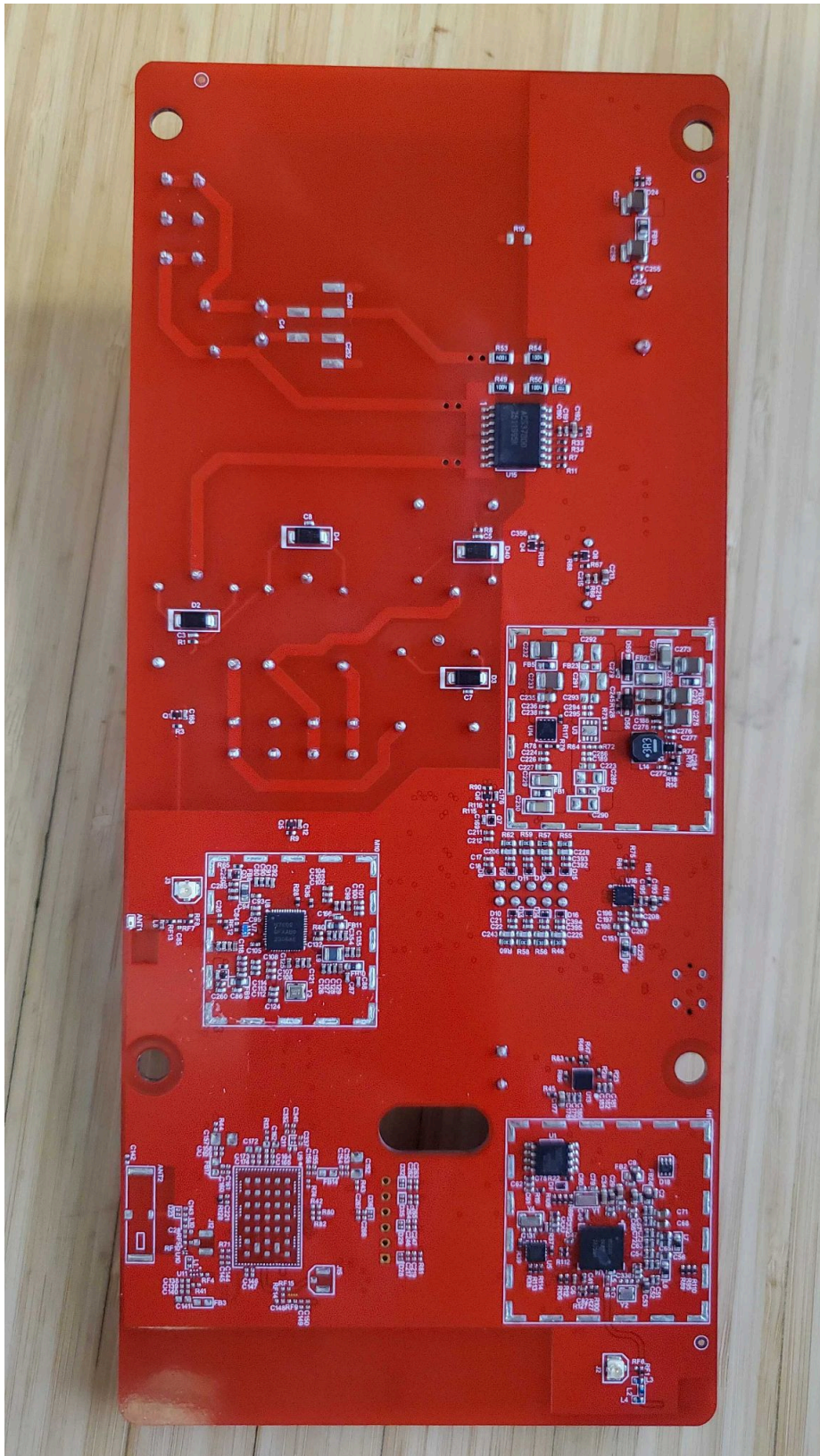
Figure 3: Big Dipper PCB-4 Bottom Without Shield
