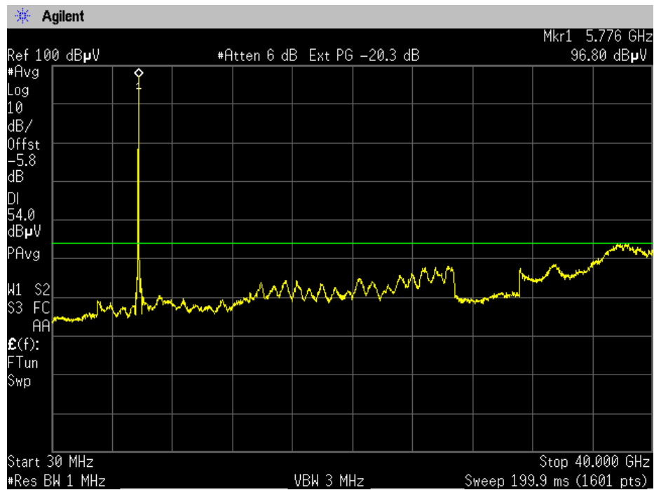
Mid Channel Restricted band 30MHz – 40 GHz – Average
