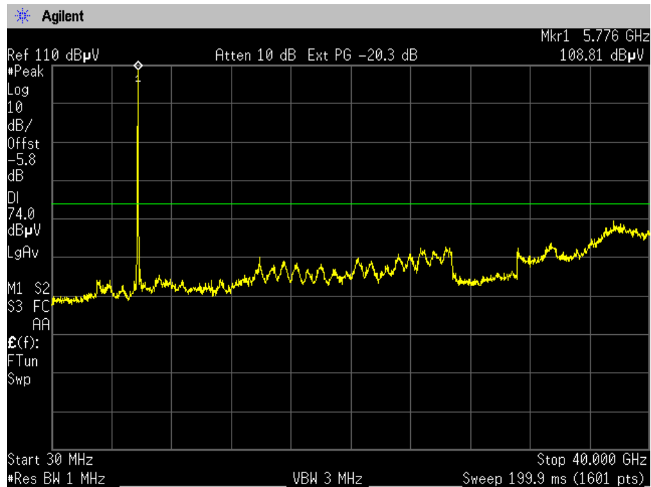
Mid Channel Restricted band 30MHz – 40 GHz - Peak
