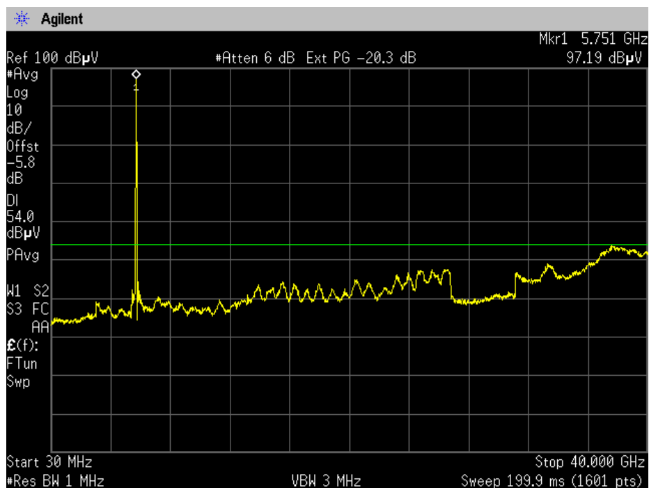
Low Channel Restricted band 30MHz – 40 GHz - AVG
