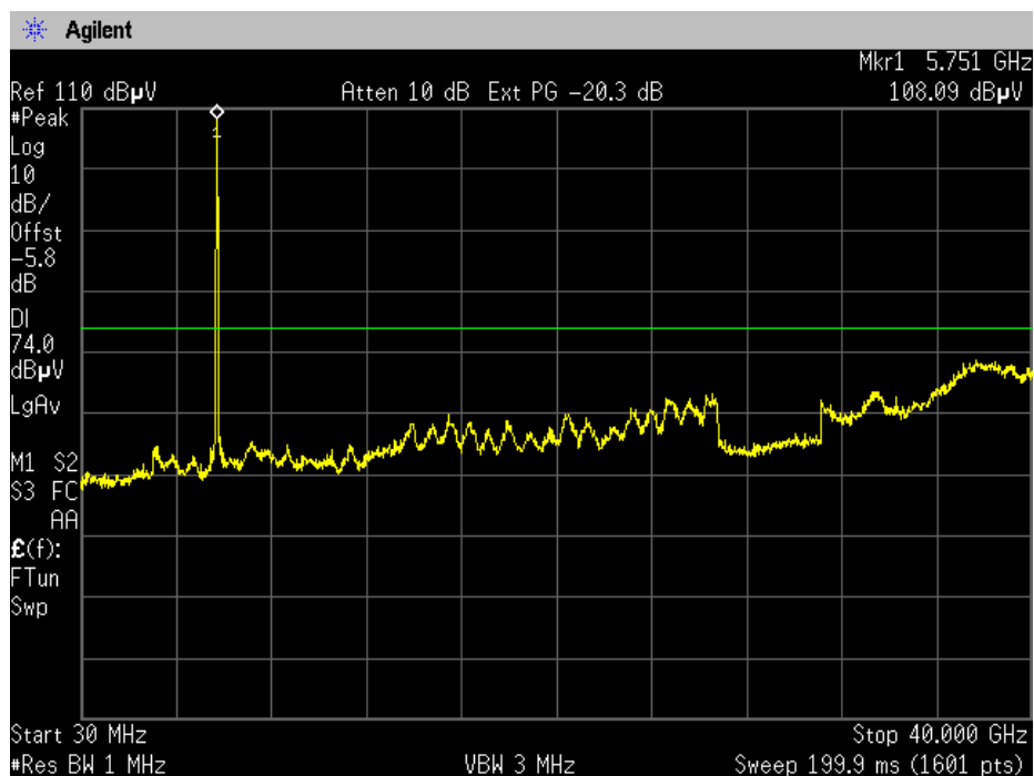
Low Channel Restricted band 30MHz – 40 GHz - Peak
