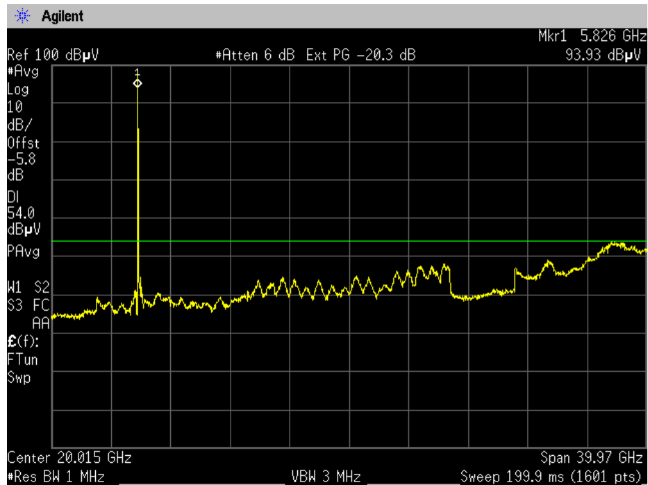
High Channel Restricted band 30MHz – 40 GHz – Average
