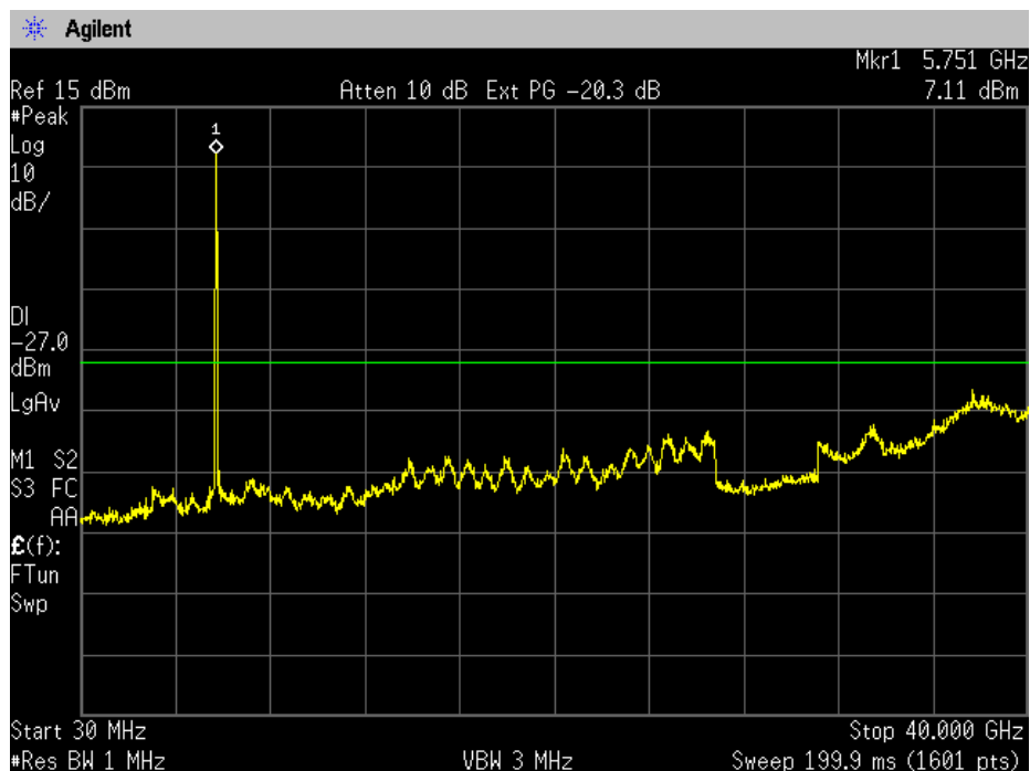
Low Channel 30MHz – 40 GHz
