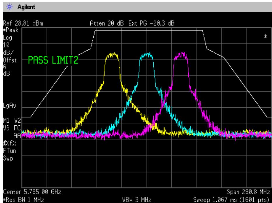
UNII-3 Mask
