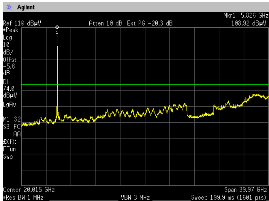
High Channel Restricted band 30MHz – 40 GHz – Peak
