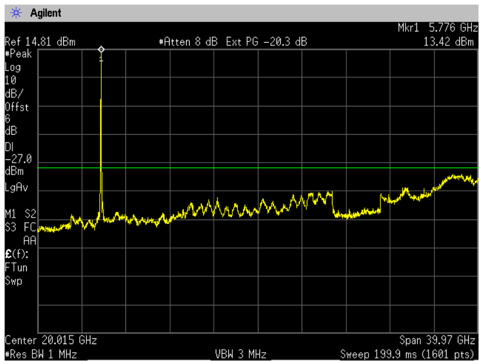
Mid Channel 30MHz – 40 GHz
