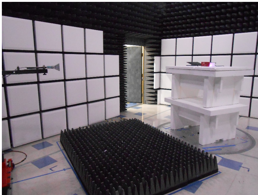
Radiated Emissions above 18 GHz
