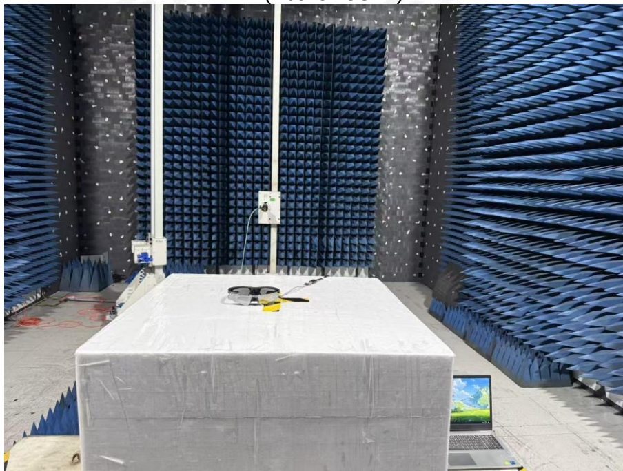
RE (Above 18GHz)
