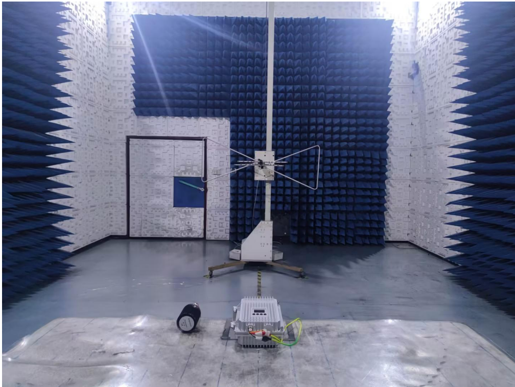
Radiated Emission Test Setup Above 1GHz (DC Power)
