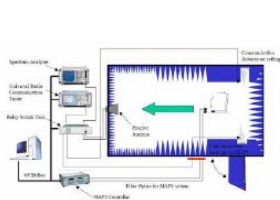
(Testing by 3D anechoic chamber)
