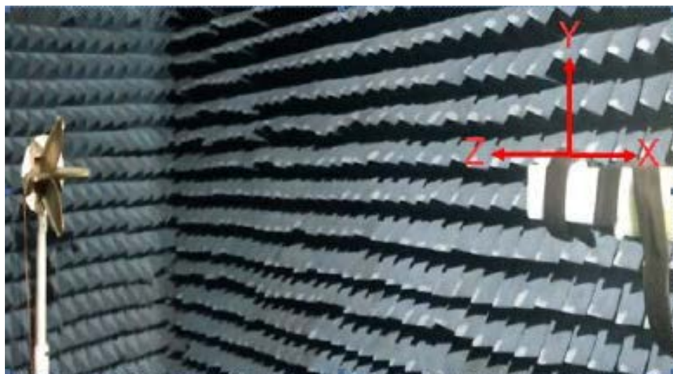
Theta axis test
