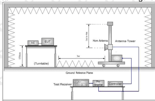
Figure 3. Above 1GHz
